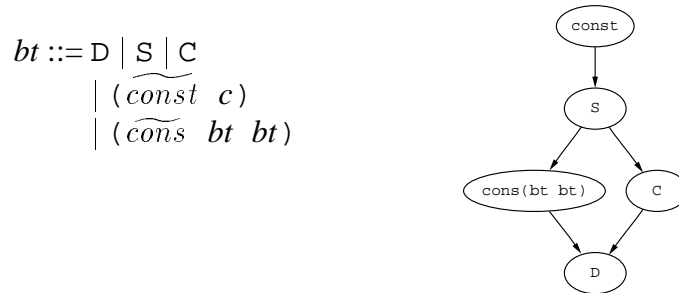
Figure 4.10: The binding time lattice. In the grammar on the left D denotes dynamic, S denotes static, C denotes cyclic, and c denotes a constant. The lattice order is illustrated on the right.
