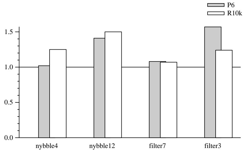
Figure 5.3: Execution time of root code automatically specialized by Nitrous normalized to time of hand-specialized code.
