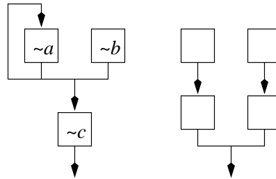
Figure 1.15: Two voices. On the left is a simple 2-in-1 synthesizer where oscillators a and b sum to modulate c as well as feeding back into a . On the right is another possibility.
