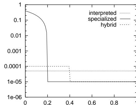
Figure 1.11: Latency of hybrid specialization and evaluation.
