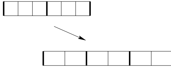
Figure 3.13: Reading a 8-bit signal and writing a 12-bit signal on a machine with 24-bit words.
