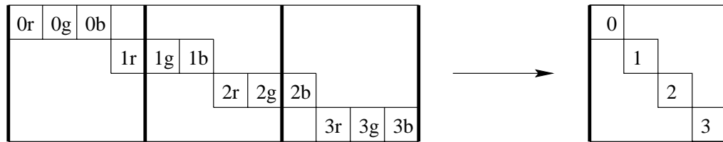
Figure 1.3: Another possible implementation packs four pixels into three words, saving 25% read-bandwidth over Figure 1.1. The code is similar to the code in Figure 1.2.
