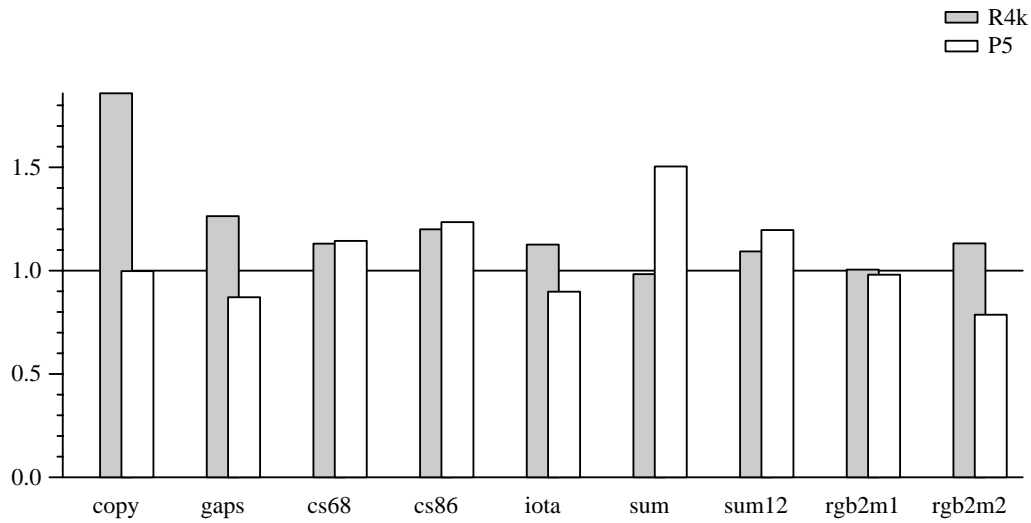
Figure 5.5: Video group. Execution time of automatically specialized by Simple normalized to time of hand-specialized code.
