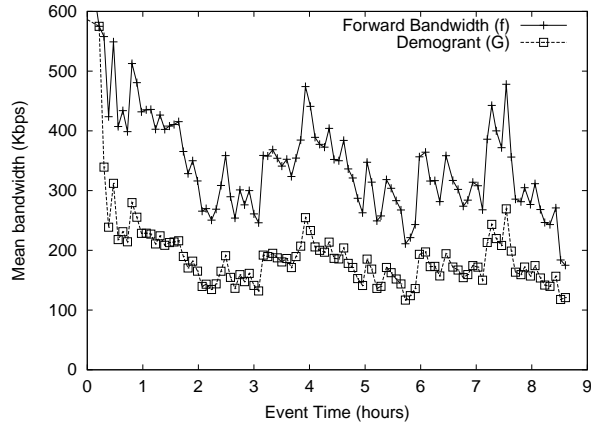
Figure 4.17: Forwarding bandwidth of peers and the resulting demogrant vs. time in the Slashdot trace simulation.
