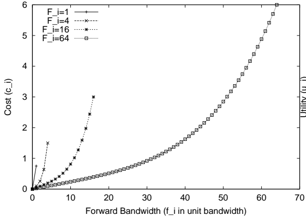
Figure 4.6: The cost as a function of forward bandwidth. The cost function depends on peer's forward capacity.
