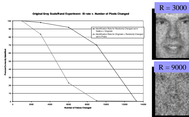
Figure 16. Eigenfaces recognition based on best matches using images perturbed by adding random noise.
