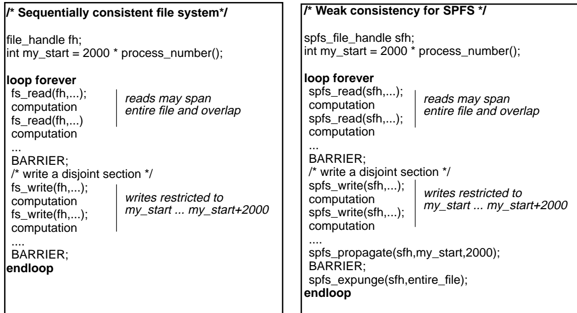
Figure 9: Data parallelism using SPFS.
