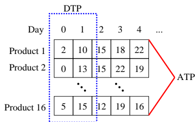
Figure 8: The strategy module instructs the agent to promise the first two days of available PCs.
