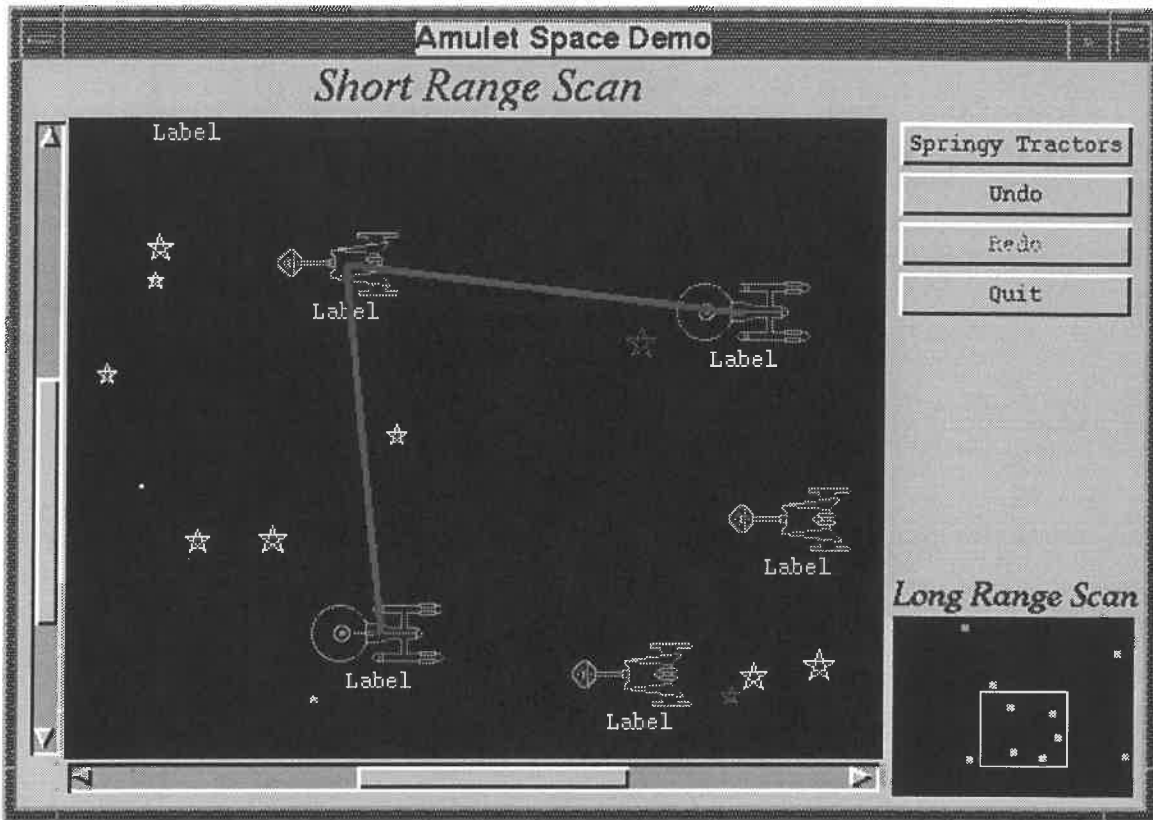
Figure 1: A sample program created using Amulet. The ships and widgets are instances created from prototypes, and constraints are used ubiquitously to keep the lines connected to the ships, compute the widget sizes, keep the window positioned appropriately based on the scroll bars, etc.
