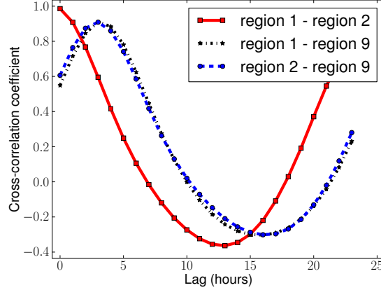
Figure 2.3: Cross correlation analysis confirms the temporal shift in access pattern over two months of data
