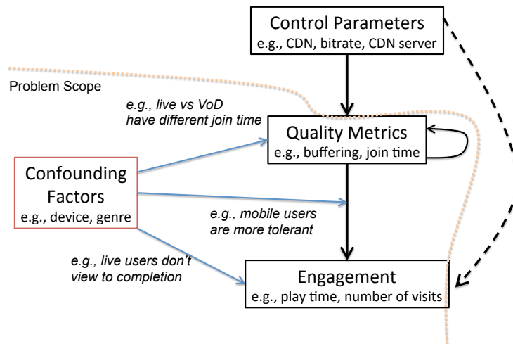
Figure 3.1: Dependencies and problem scope
