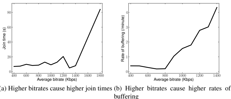
Figure 3.3: The quality metrics are interdependent on each other
