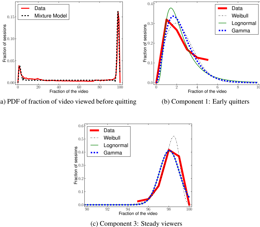
Figure 2.10: Distribution of the fraction of video viewed for VOD
