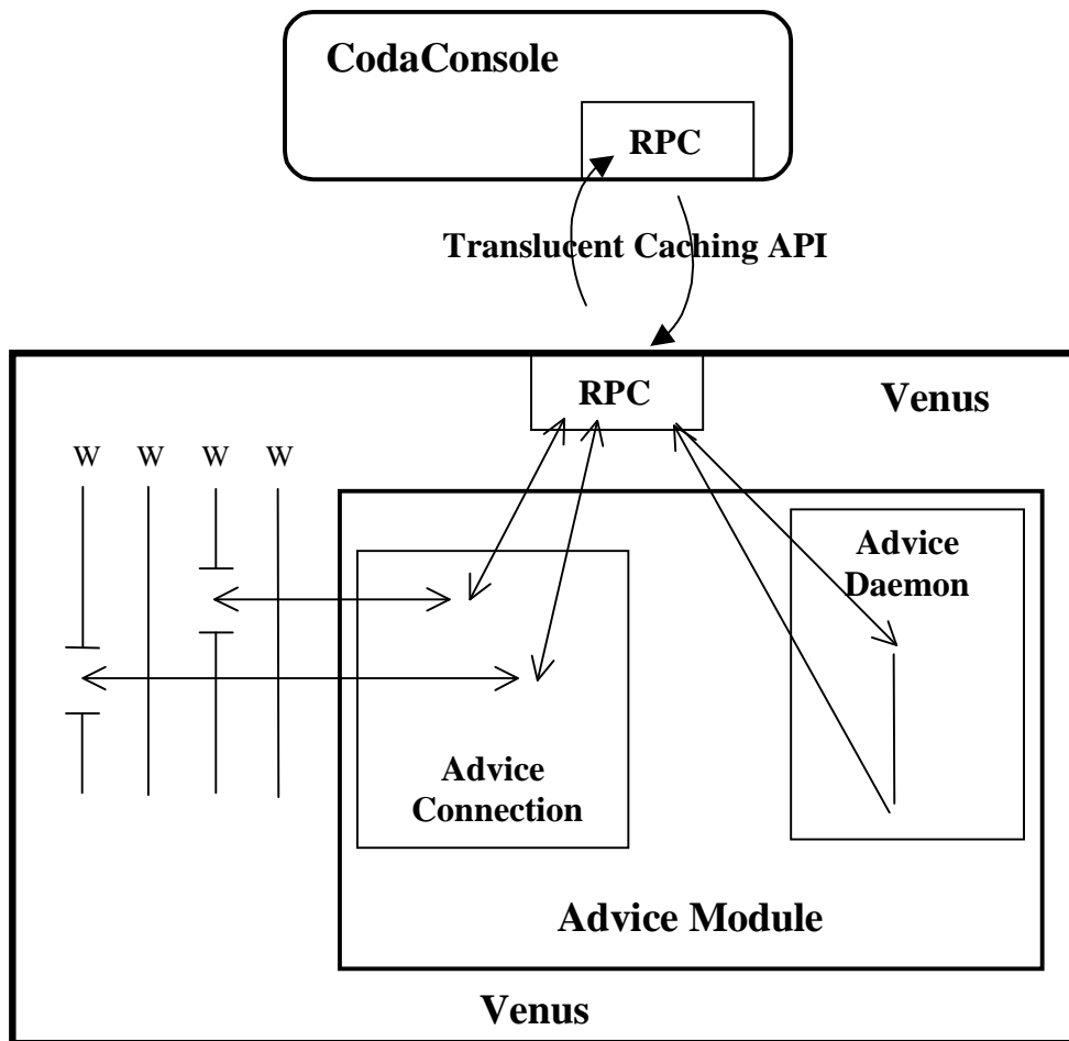
Figure 5.5: Relevant Venus Internals
