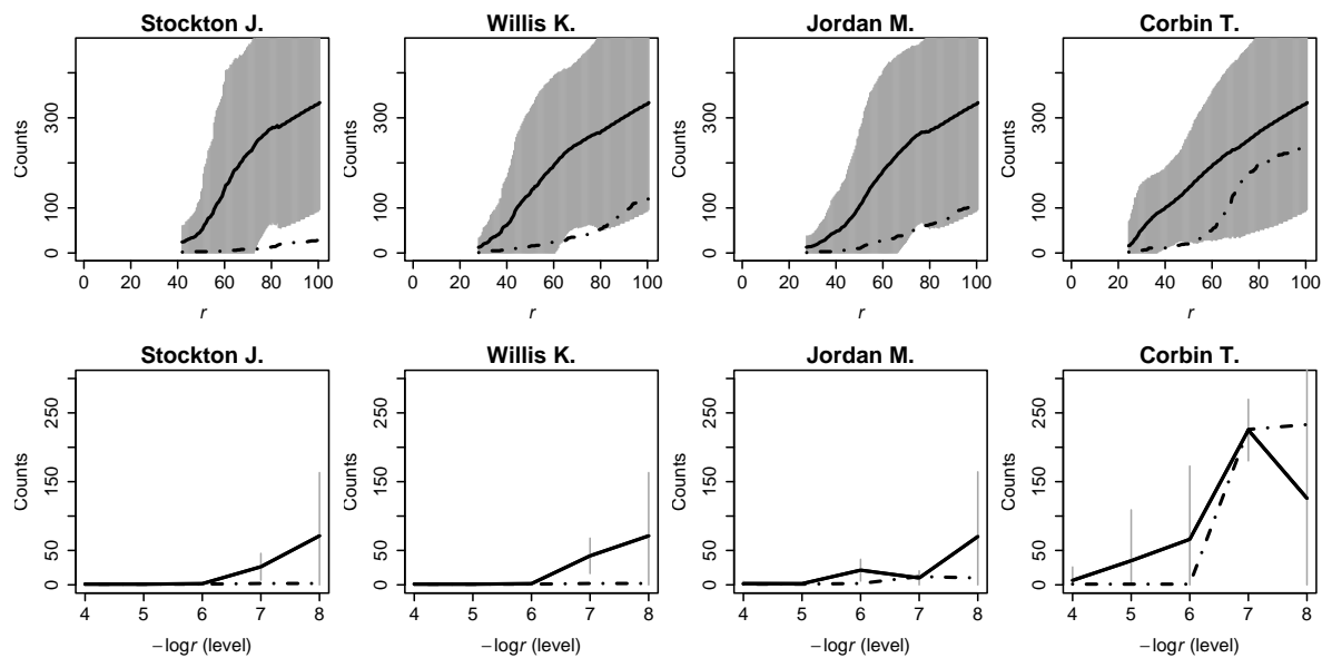
Figure 14: NBA, LOCI plots.
