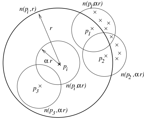
Figure 3: Definitions for n and \hat{n} —for instance n(p_i, r) = 4 , n(p_r, \alpha r) = 1 , n(p_1, \alpha r) = 6 and \hat{n}(p_i, r, \alpha) = (1 + 6 + 5 + 1)/4 = 3.25 .
