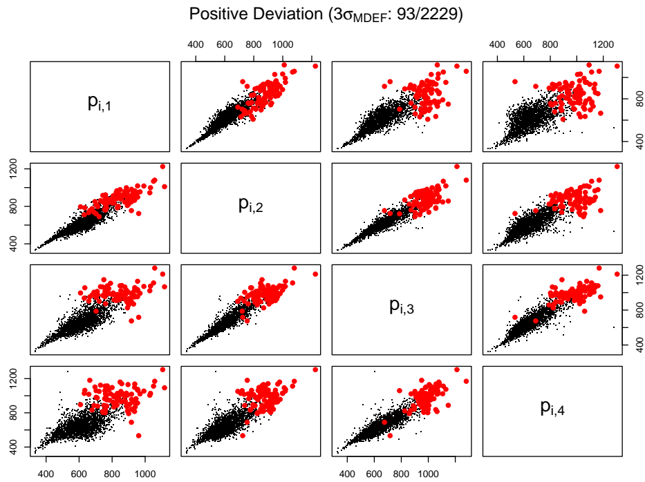
Figure 15: NYWomen, results, LOCI ( \hat{n} = 20 to full radius) and aLOCI (bottom; 6 levels, l_\alpha = 3 , 18 grids).
