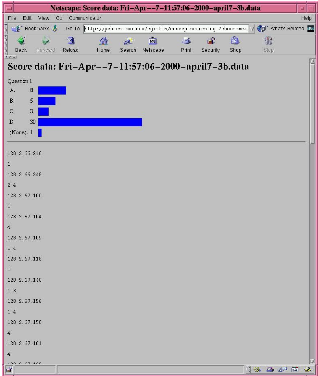
Figure 17: Example of display of saved concept test data.
