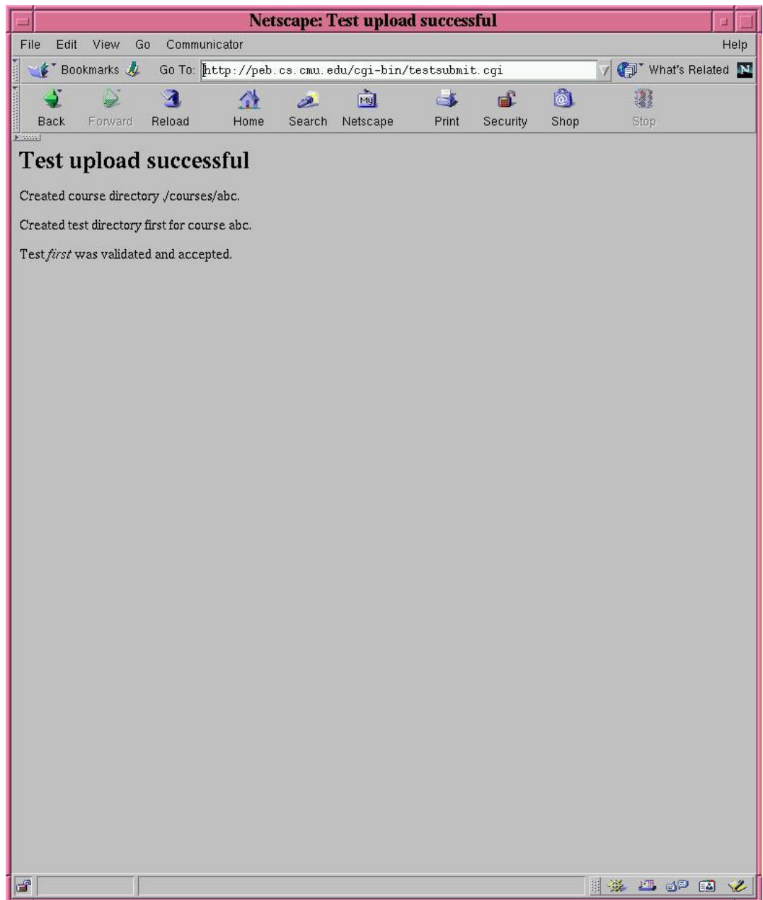
Figure 12: Page after instructor has successfully uploaded the test
