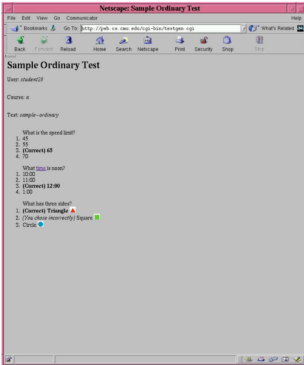
Figure 10: Page for an ordinary test, after a response has been submitted
