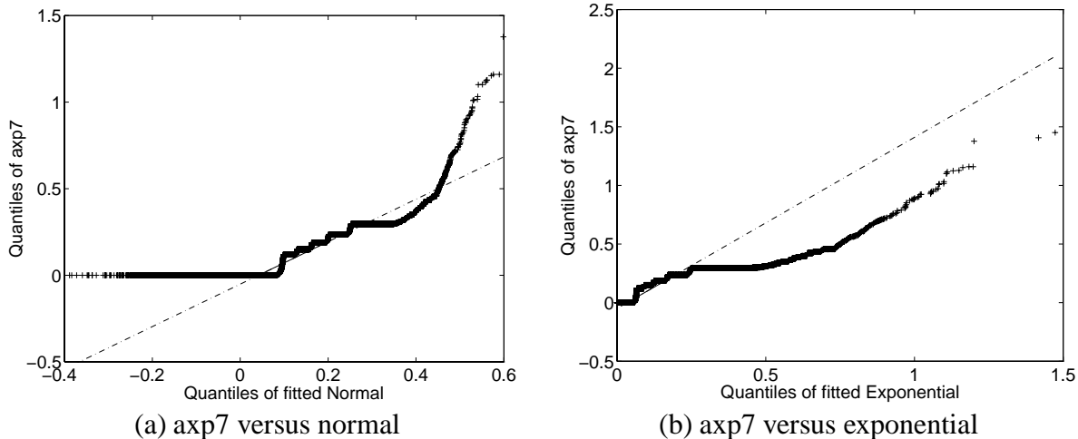
Figure 9: Quantile-quantile plots for axp7 trace of August 19, 1997.
