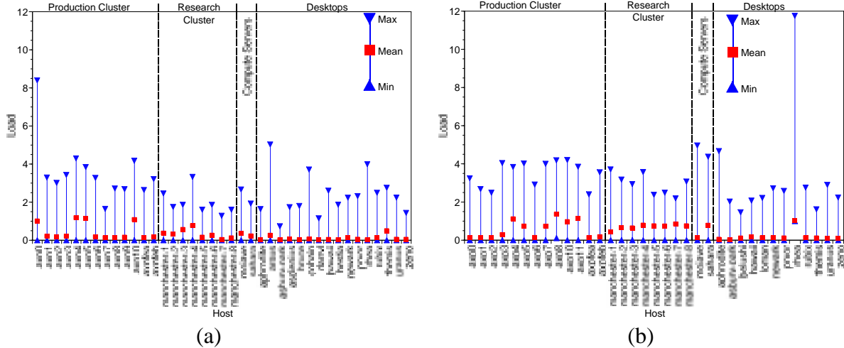
Figure 6: Minimum, maximum, and mean load: (a) August, 1997 traces, (b) March, 1998 traces.
