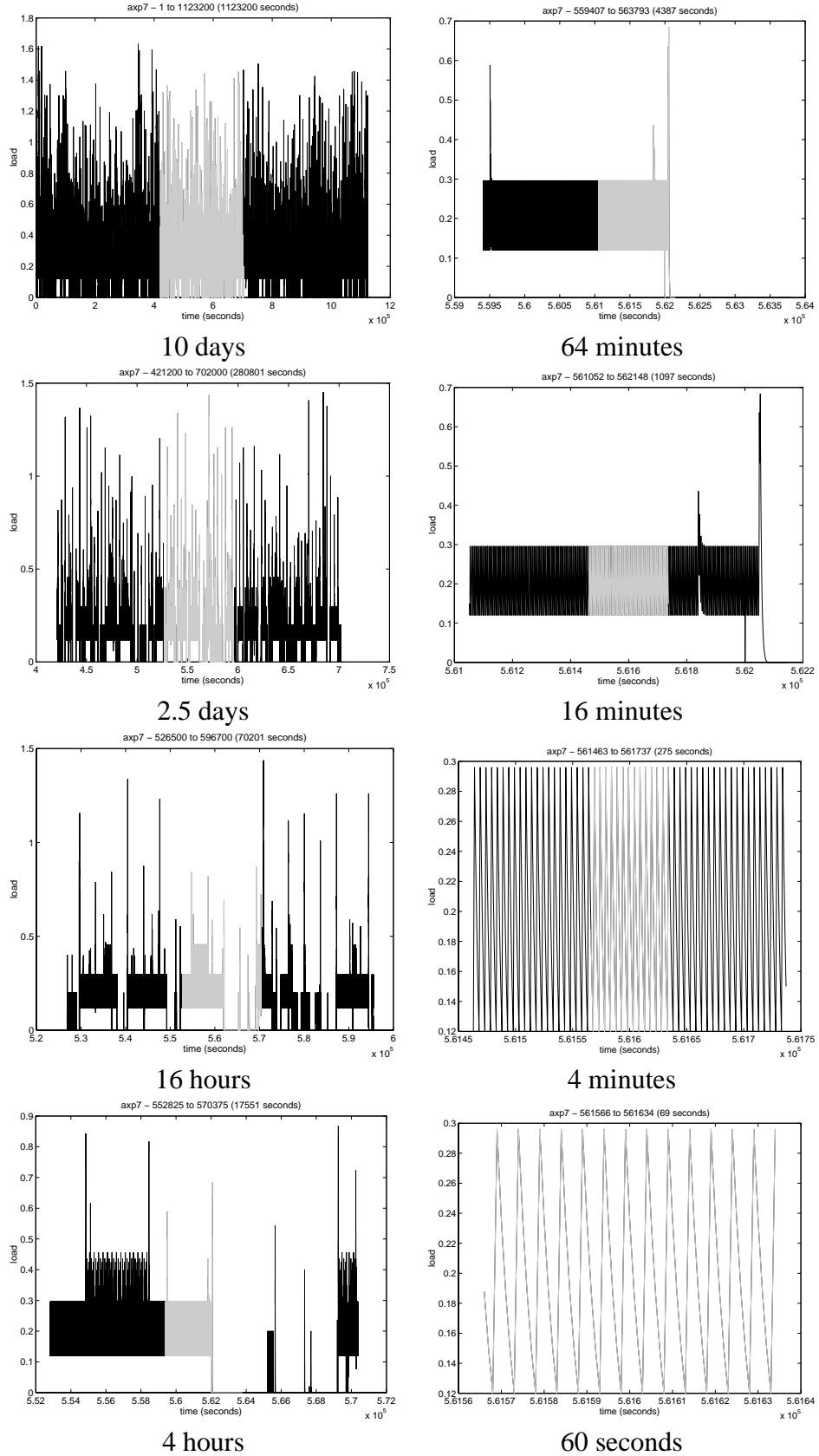
Figure 11: Visual representation of self-similarity. Each graph plots load versus time and “zooms in” on the middle quarter
