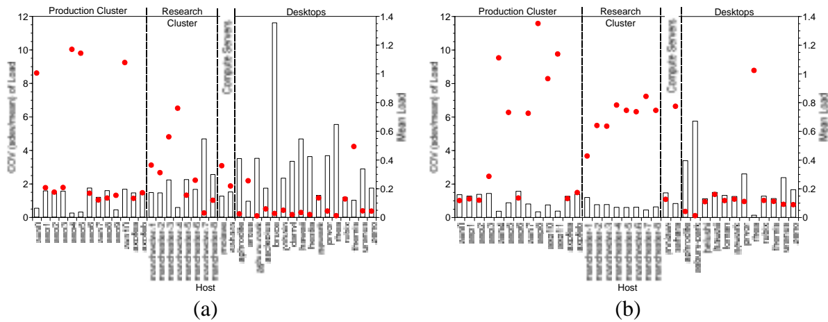
Figure 5: COV of load and mean load: (a) August, 1997 traces, (b) March, 1998 traces.
