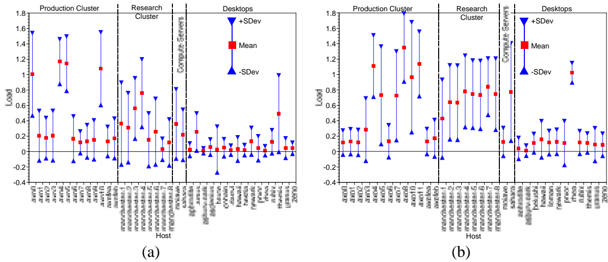
Figure 4: Mean load +/- one standard deviation: (a) August, 1997 traces, (b) March, 1998 traces.
