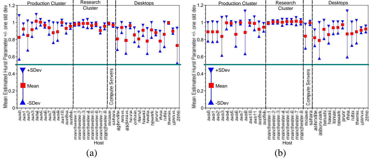
Figure 13: Hurst parameter estimates (mean of four point estimates and standard deviation) : (a) August, 1997 traces, (b) March, 1998 traces.
