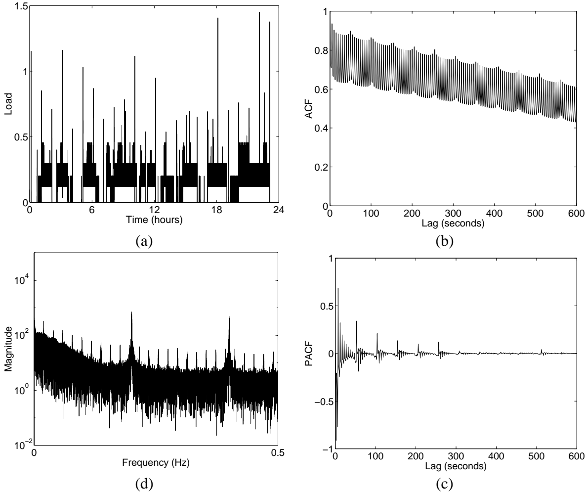
Figure 10: Time series analysis of axp7 load trace collected on August 19, 1997: (a) Load trace, (b) Autocorrelation function to lag 600 (10 minutes), (c) Partial autocorrelation function to lag 600 (10 minutes), (d) Periodogram.
