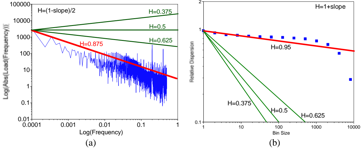
Figure 12: Meaning of the Hurst parameter: (a) Frequency domain interpretation using power spectral analysis, (b) Effect of increased smoothing using dispersional analysis.
