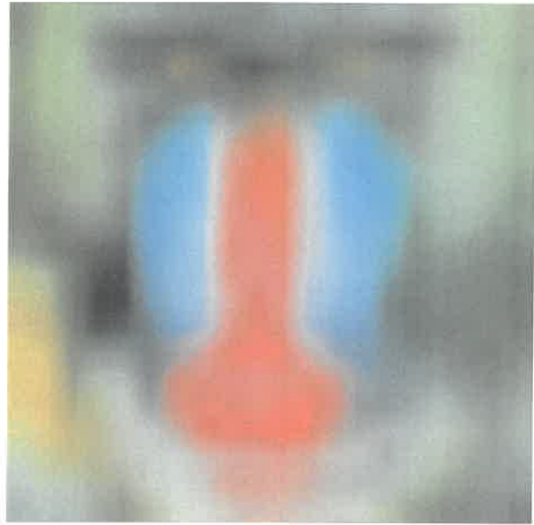
Figure 24: Mandrill approximated with Gouraud shaded triangles created by subsampling on a uniform 20×20 grid (400 vertices).
