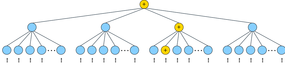
Figure 3.4: A learning problem where exponential rates are not achievable. The instance space is an infinite-depth tree. The target labels nodes along a single infinite path as +1, and labels all other nodes -1. For any \phi(\epsilon) = o(1/\epsilon) , when the number of children and probability mass of each node at each subsequent level are set in a certain way, label complexities of o(\phi(\epsilon)) are not achievable for all targets.
