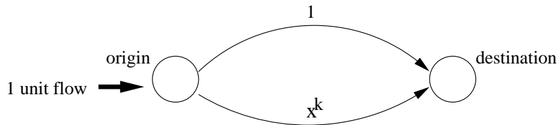
Figure 1: A simple example of bad coordination ratio when latency gradient is unbounded
