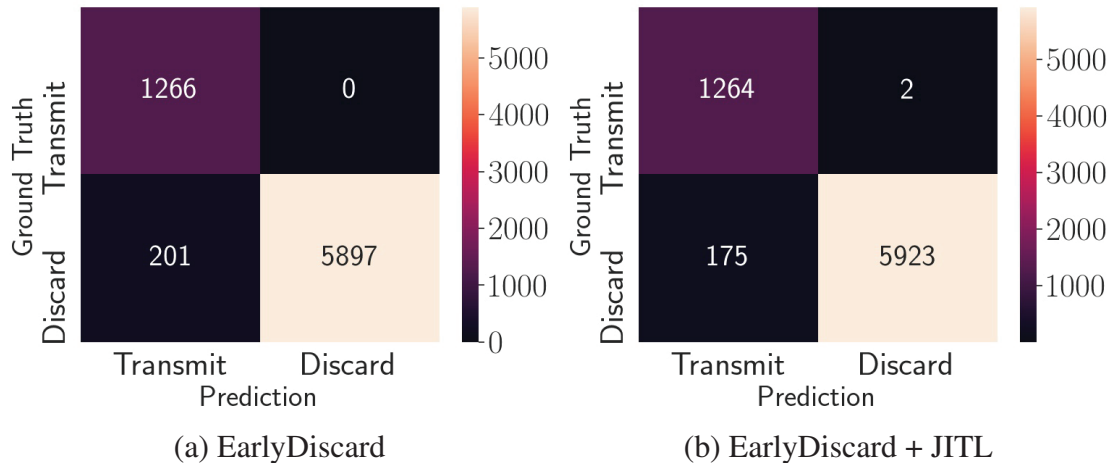
Figure 3.12: JITL Confusion Matrix
