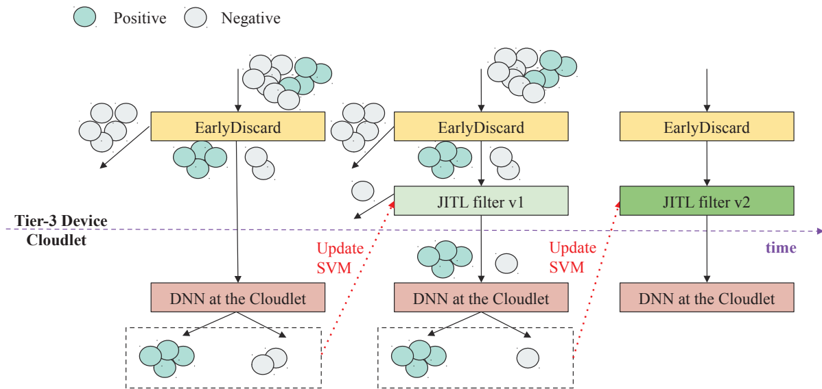
Figure 3.7: JITL Pipeline
