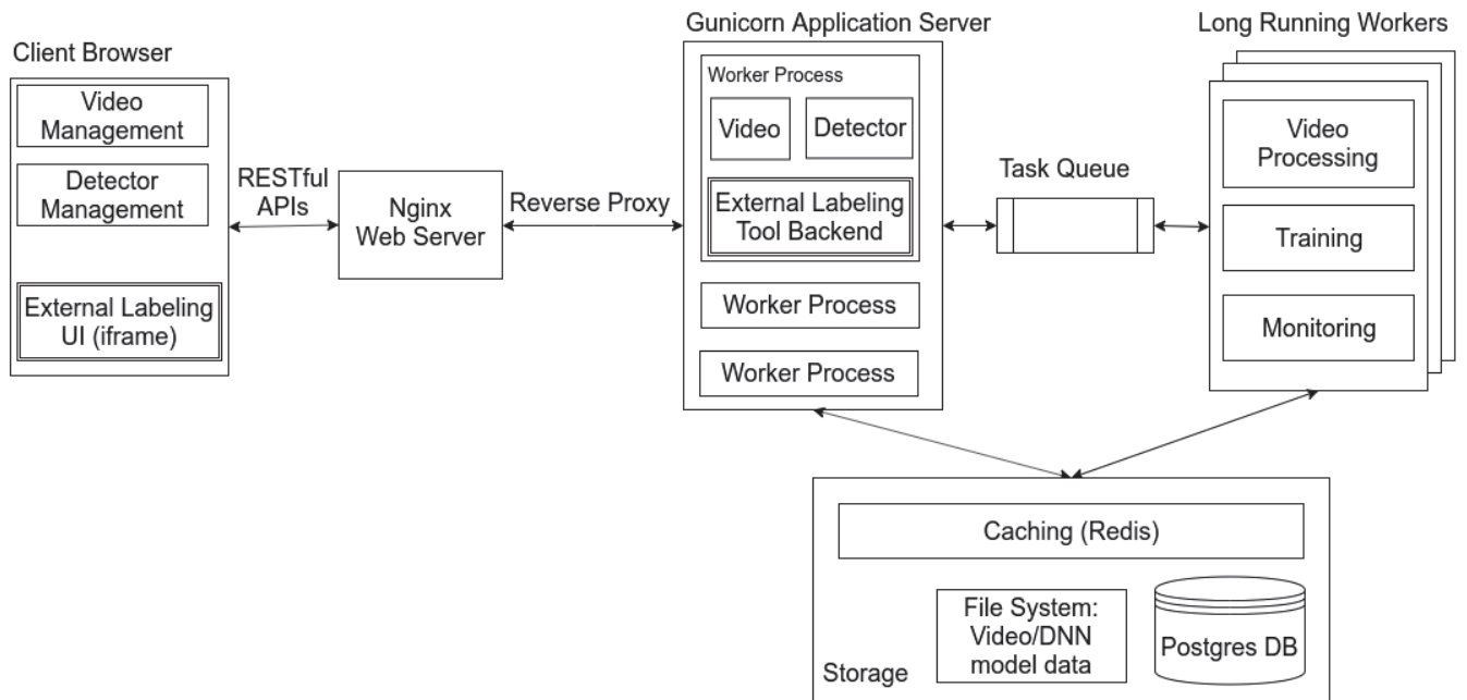
Figure 6.8: OpenTPOD Architecture
