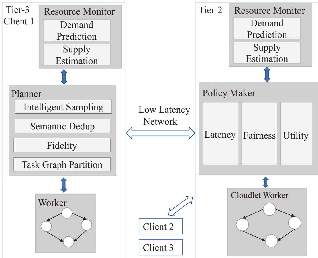
Figure 4.1: Adaptation Architecture
