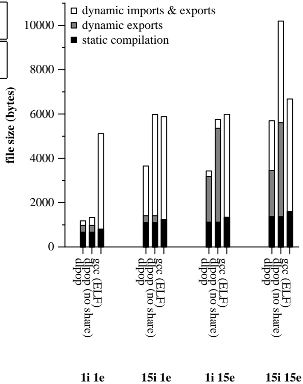
Figure 7: Comparing the space overhead of DLpop, DLpop without type representation sharing, and Dlopen/ELF for some microbenchmarks.
