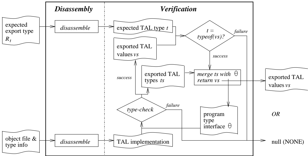
Figure 1: The implementation of load
