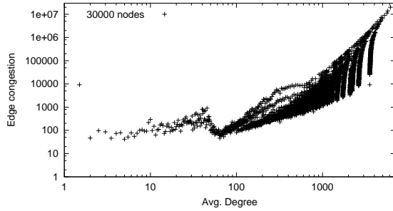
Figure 13: Edge Congestion versus the average degree of the nodes incident on the edge (any-2-any model with shortest path routing). The congestion is higher on edges with a high average degree.
