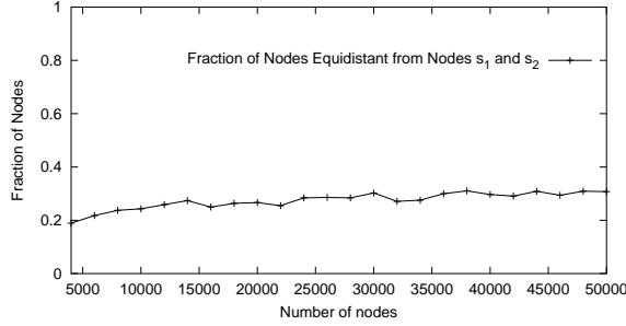
Figure 2: Fraction of shortest path trees that do not contain the edge e^* .
