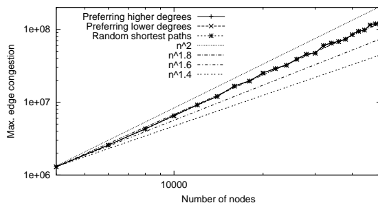
Figure 8: Edge congestion with shortest path routing and any-2-any communication, with \alpha = 1.23 . The figure plots the three different variations of breaking ties in shortest path routing.
