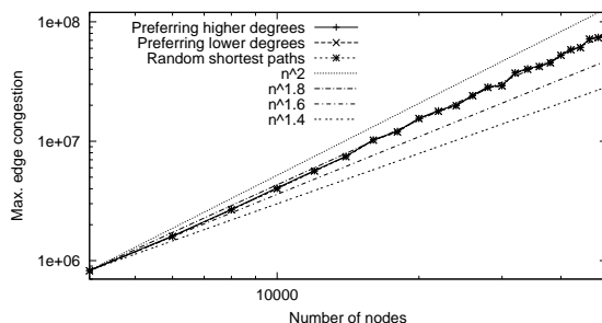
Figure 9: Edge congestion with shortest path routing and leaf-2-leaf communication, with \alpha = 1.23 . The figure plots the three different variations of breaking ties in shortest path routing.
