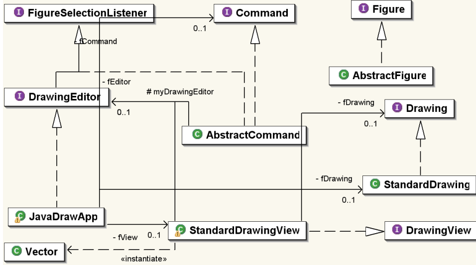
Figure 1: MicroDraw: UML class diagram.
