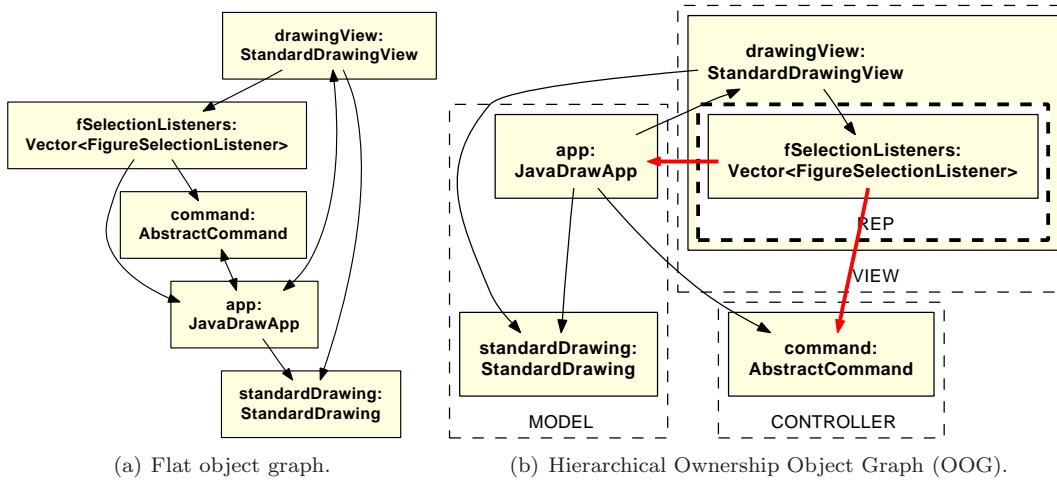
(a) Flat object graph.
