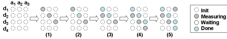
Figure 3: Example of the scheduling algorithm
