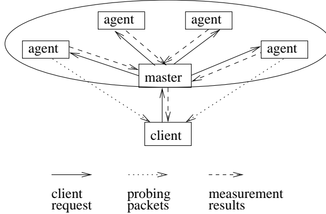
Figure 2: Emodis system architecture
