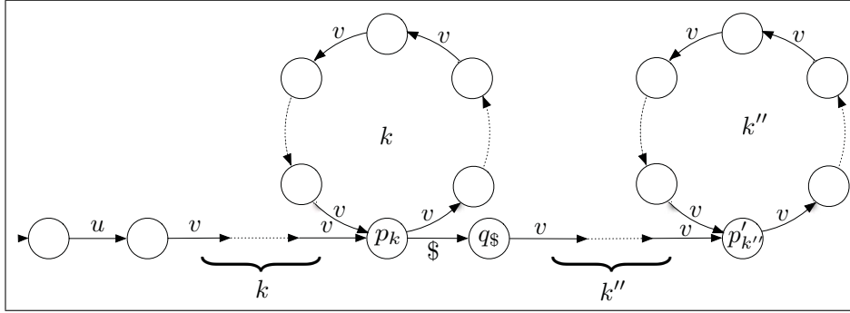
Figure 4: Proof Diagram.
