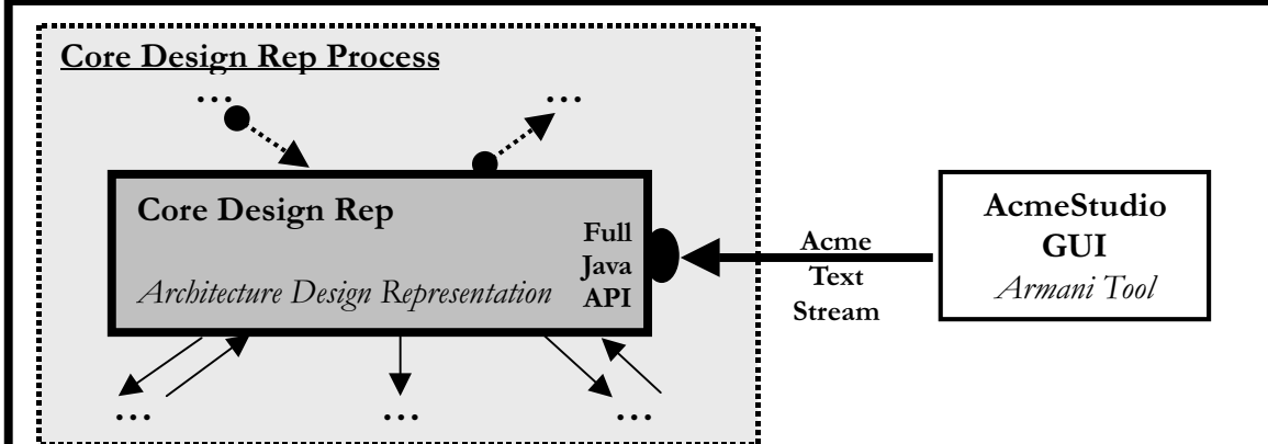
Figure 5.3b: Using a streamed Acme Text connector to integrate the AcmeStudio GUI with the Armani core design environment infrastructure.
