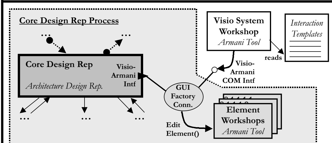
Figure 5.3c: Integrating the Visio-based, fine-grained configurable Armani interface with the GUI Factory connector and configurable editing workshops.
