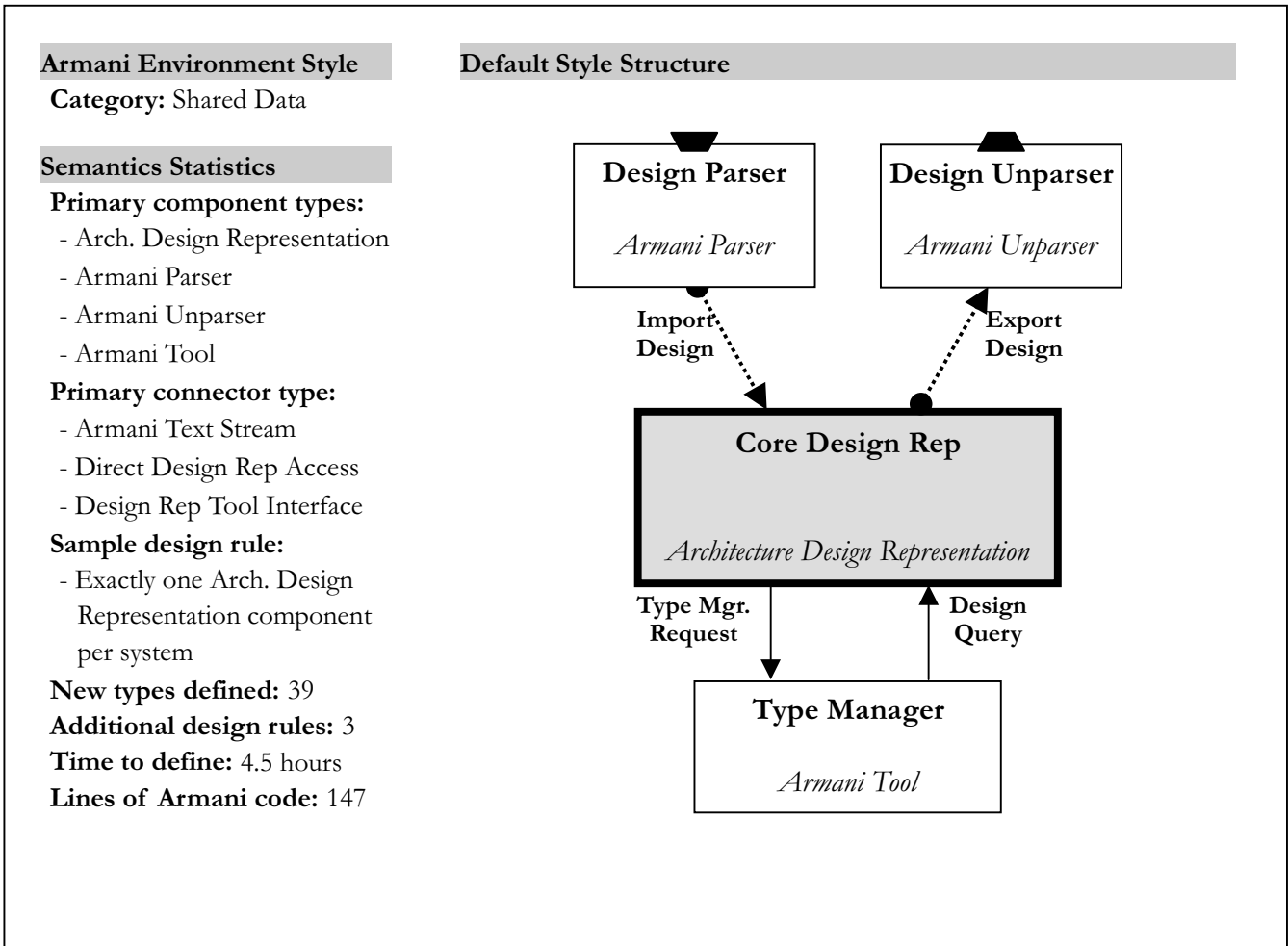
Figure 7.9: Overview of the Armani Environment Style
