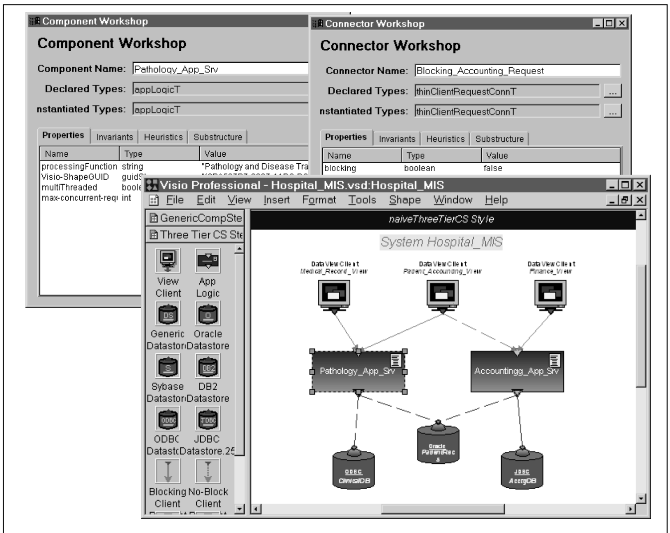
Figure 2.4: The Armani design environment customized after extending the naive client-server style to support the three-tier client-server style
