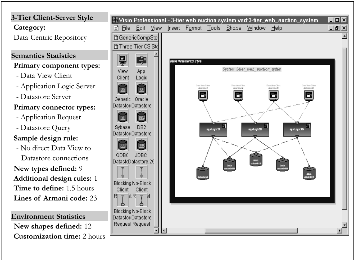
Figure 7.6: Overview of the Three-Tier extension to the Naïve Client-Server style and environment
