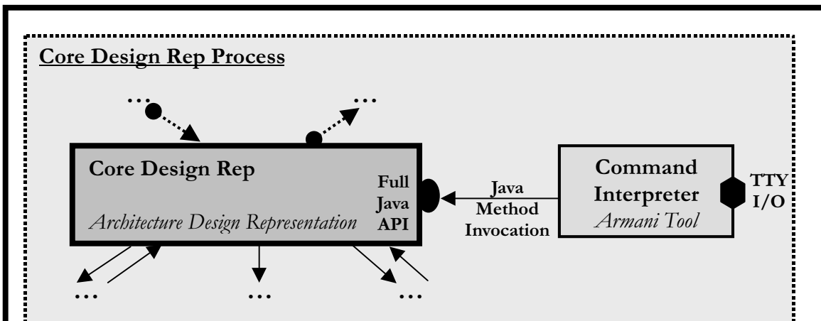
Figure 5.3a: Integrating a command interpreter user interface with a direct Java method invocation connector
