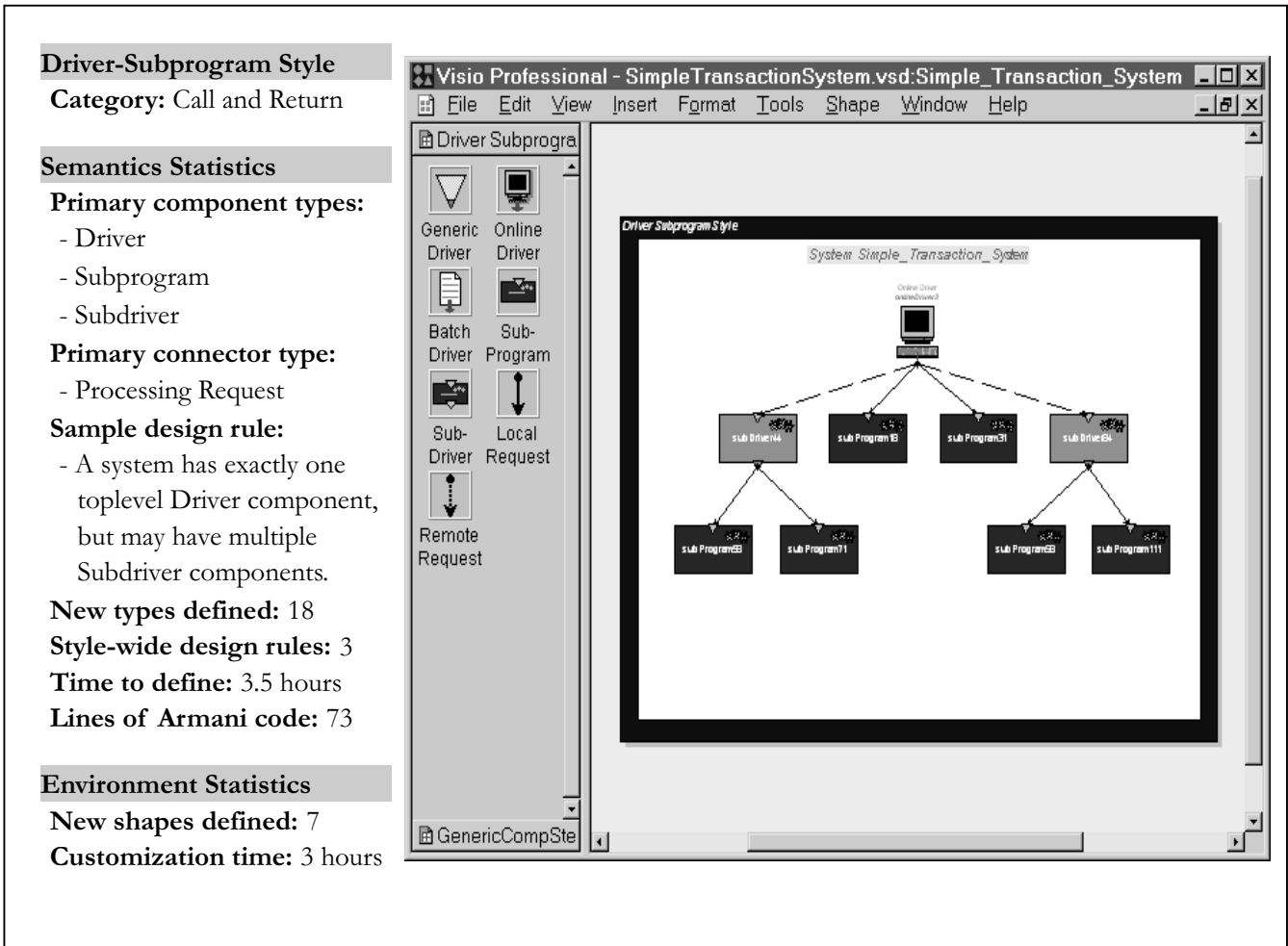
Figure 7.7: Overview of the Driver-Subprogram style and environment
