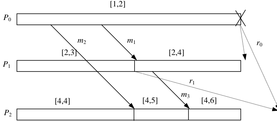
Figure 14. Exponential rollbacks.
