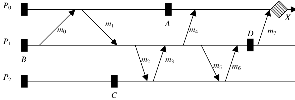
Figure 13. Optimistic logging.
