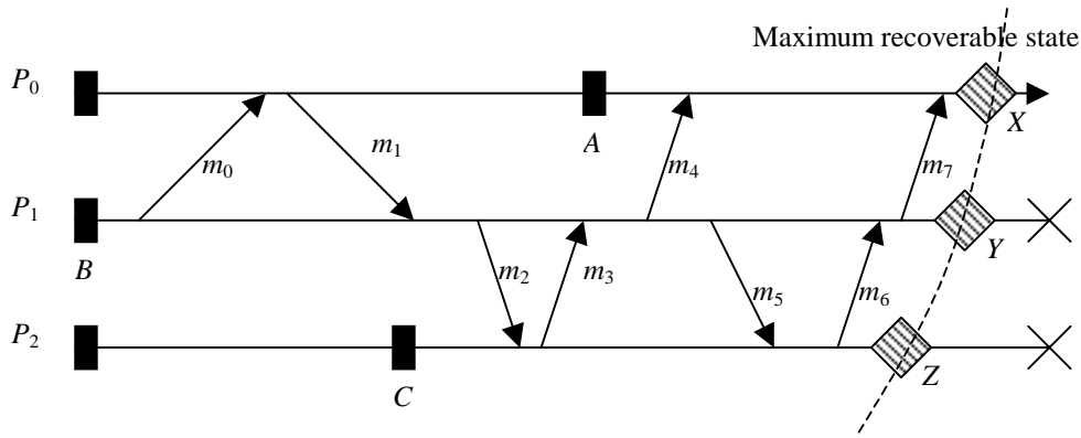
Figure 12. Pessimistic logging.
