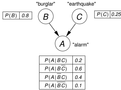
(a) Bayesian network.
