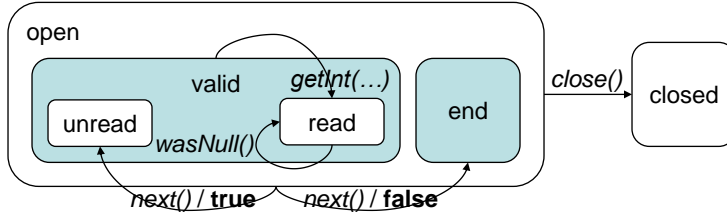
Figure 1: Simplified JDBC ResultSet protocol. Rounded rectangles denote states refining another state. Arches represent method calls, optionally with return values.
