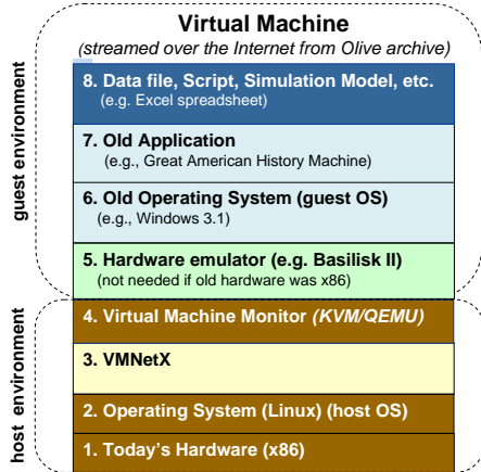
Figure 5: Abstract Olive Client Structure
