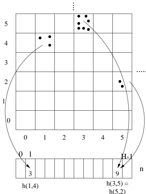
Figure 2: Density approximation by hashing
