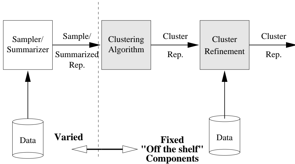
Figure 6: Clustering framework
