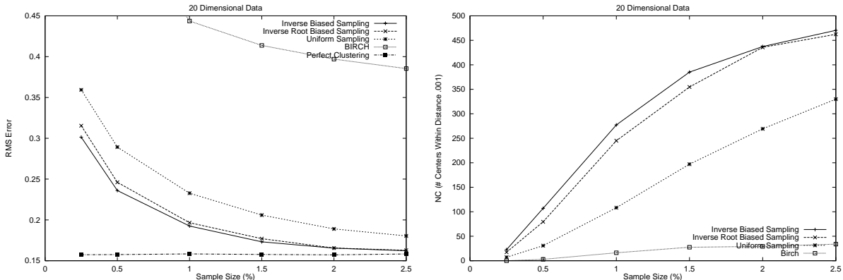
Figure 9: Zipf sizes ( d=20 ): RMS Error predicted and NC for the same experiment
