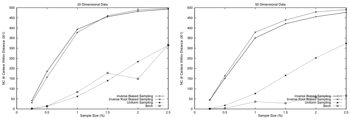
Figure 10: OneBig sizes ( d=20/50 ): Ideal case for density biased sampling
