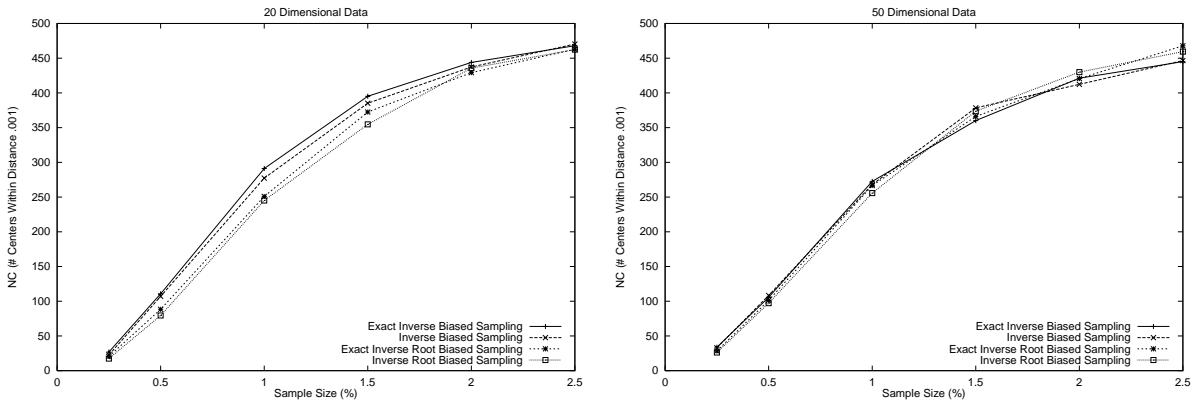
Figure 13: Zipf sizes ( d=20/50 ): Collisions only cause minor differences
