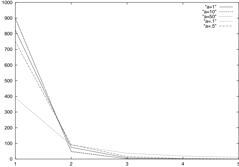
Figure 1: The expectations of size indices with various parameter values of \alpha
