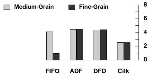
Figure 17: Speedups for the tree-building phase of Barnes Hut (for 1M particles). The phase involves extensive use of locks on cells of the tree to ensure mutual exclusion. The Pthreads-based schedulers (all except Cilk) support blocking locks. “DFD” does not result in a large scheduling granularity due to frequent suspension of the threads on locks; therefore, its performance is similar to that of “ADF”. Cilk [20] uses a pure work stealer and supports spin waiting locks. For this benchmark, the single-processor execution time on Cilk is comparable with that on the Pthreads-based system.
