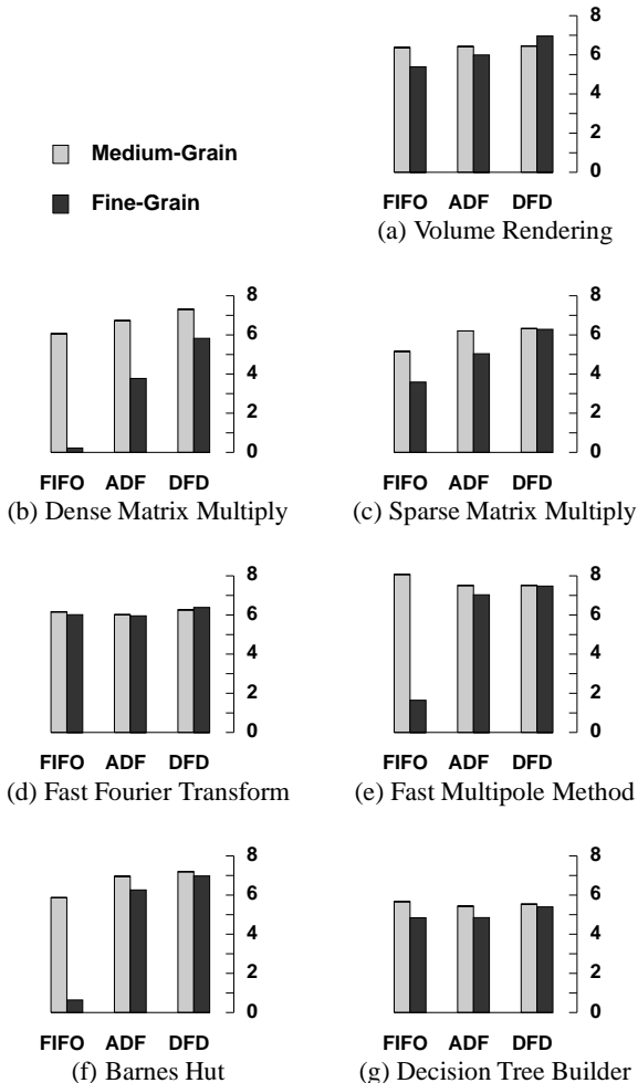
Figure 12: Speedups on 8 processors with respect to single-processor executions for the three schedulers (the original “FIFO”, the depth-first “ADF”, and the new “DFD” or DFDeques ) at both medium and fine thread granularities, with K = 50,000 bytes. Performance of “DFD-inf” (or DFDeques ( \infty )), being very similar to that of “DFD”, is not shown here. All benchmarks were compiled using cc -fast -xarch=v8plusa -xchip=ultra -xtarget=native -xO4 .
