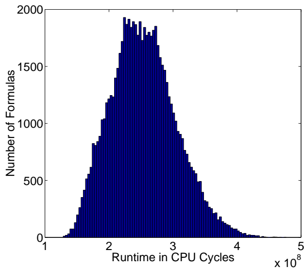
Figure 1.1: Histogram of runtimes for 70,376 different FFT(2^{18}) formulas.
