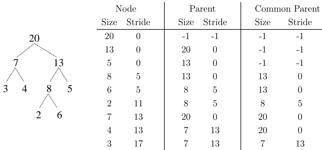
Figure 7.2: Example node features for all of the nodes in the given WHT split tree.
