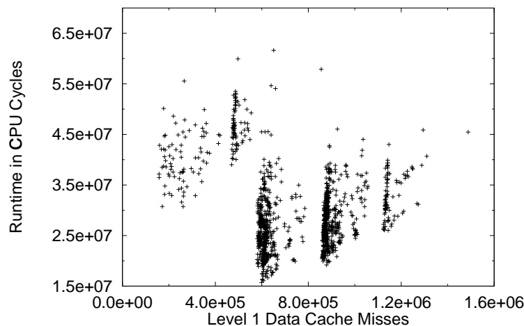
Figure 6.5: Runtimes vs. cache misses for entire WHT(2^{18}) formulas on a Sun.
