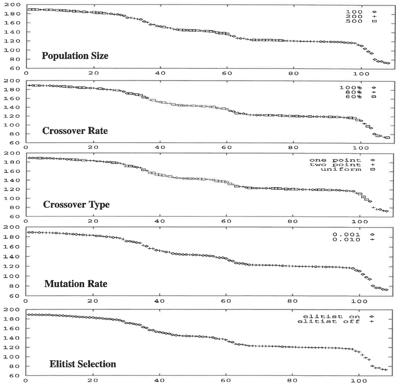
Figure 3: The 108 GA runs. Each point represents the average best evaluation (over 60 runs) of a GA. The parameters of the GA are shown in the graphs. The runs are sorted from best (left) to worst (right). The Y-Axis is the performance of the algorithm, the X-Axis is the test number.
