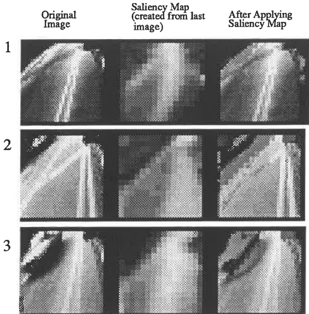
Figure 3: Images before and after applying the saliency map. In images 1 the edge of the road is bright enough to cause distractions. In 2, the two lane markings may confuse the lane tracker, and cause it oscillate between the lane markings. In 3, a passing car is removed from the image.
