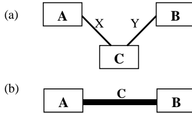
Fig. 8. Component or connector?
