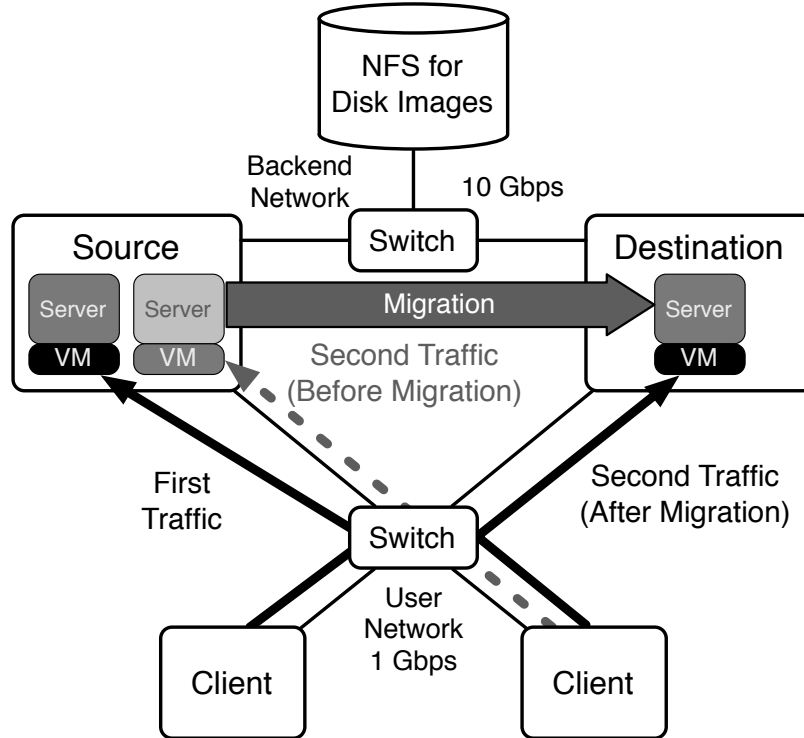
Figure 9: Experiment Set-Up
