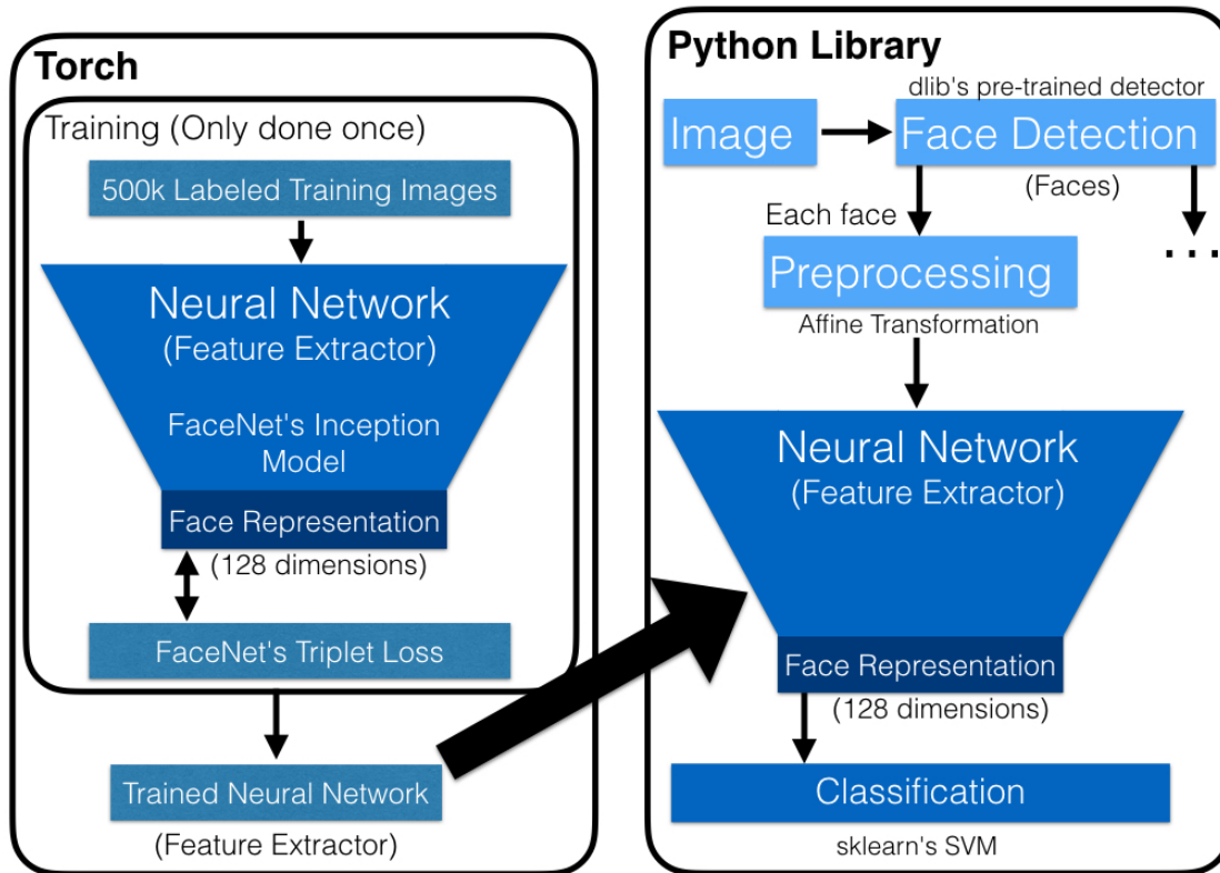
Figure 4: OpenFace's project structure.
