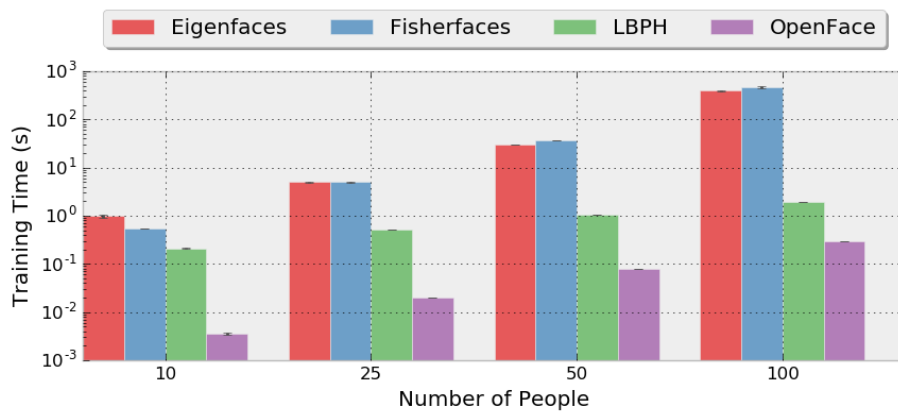
(b) Training times.
