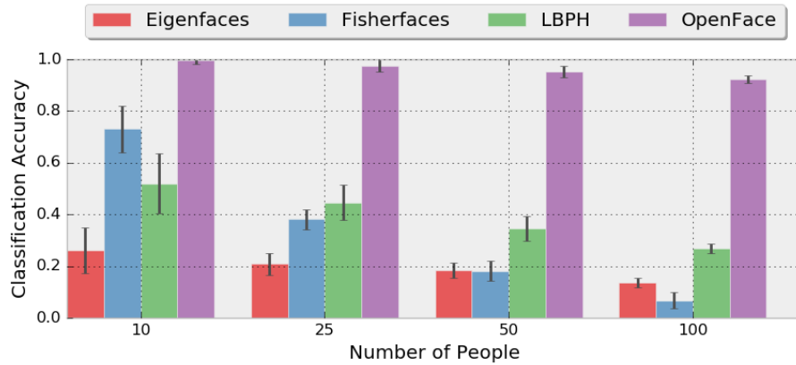
(a) Classification accuracy.
