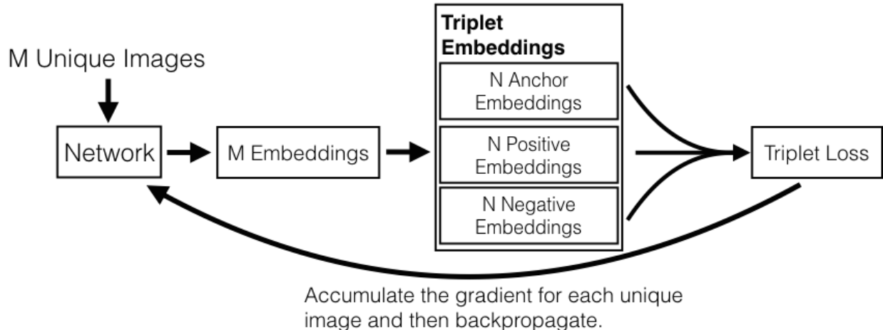
Figure 6: OpenFace’s end-to-end network training flow.
