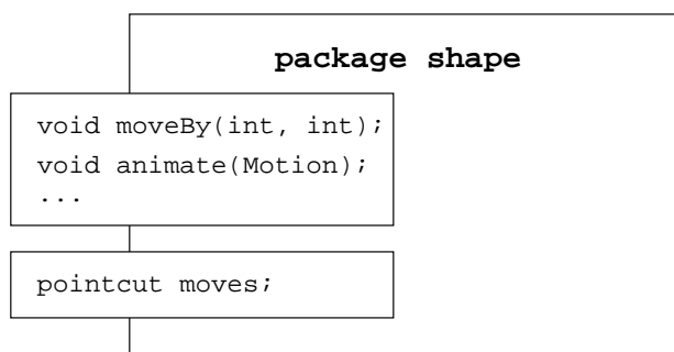
Figure 1: A conceptual view of Open Modules. The shape module exports two functions and a pointcut. Clients can place advice on external calls to the exported functions, or on the exported pointcut, but not on calls that are internal to the module.
