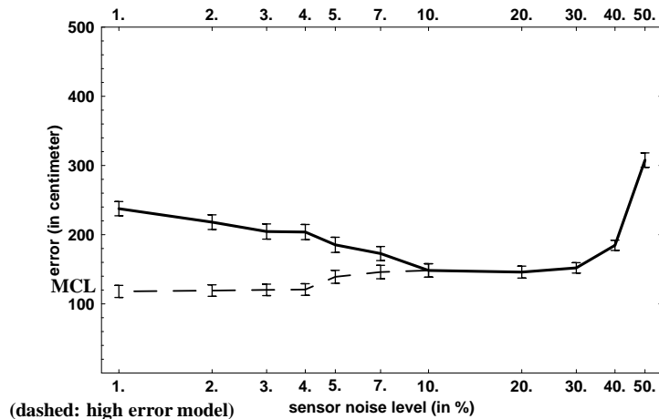
Figure 10: Solid curve: error of MCL after 100 steps, as a function of the sensor noise. 95% confidence intervals are indicated by the bars. Notice that this function is not monotonic, as one might expect. Dashed curve: Same experiment with high-error model.
