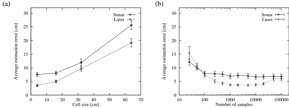
Figure 7: (a) Accuracy of grid-based Markov localization using different spatial resolutions. (b) Accuracy of MCL for different numbers of samples (log scale).
