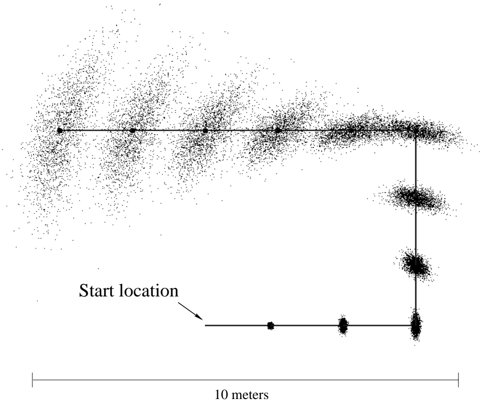
Figure 2: Sampling-based approximation of the position belief for a robot that only measures odometry. The solid line displays the actions, and the samples represent the robot's belief at different points in time.
