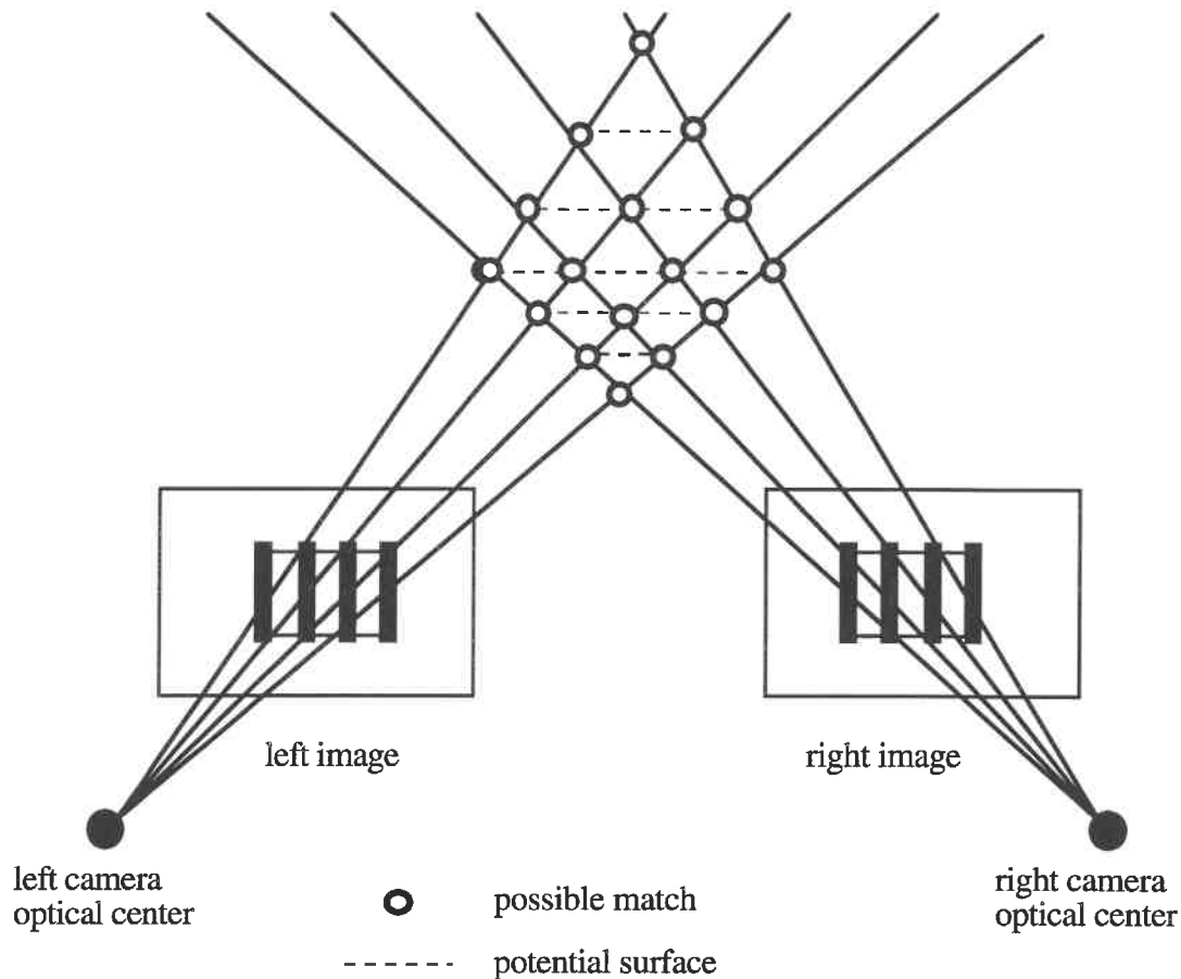
Figure 2: The projection of two images containing a repetitively textured object into 3D space. Notice the potential surface with the highest number of matches is the correct surface.
