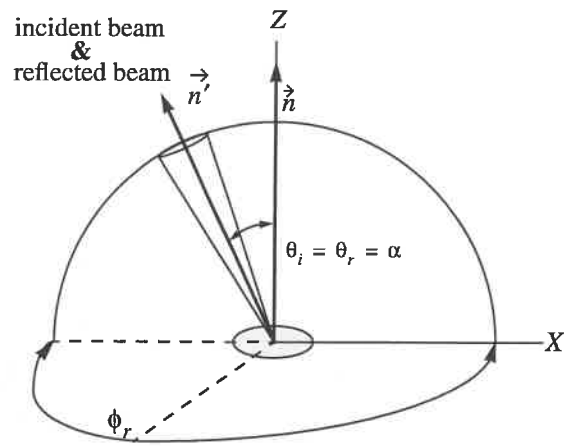
Figure 10 Simplified geometry
