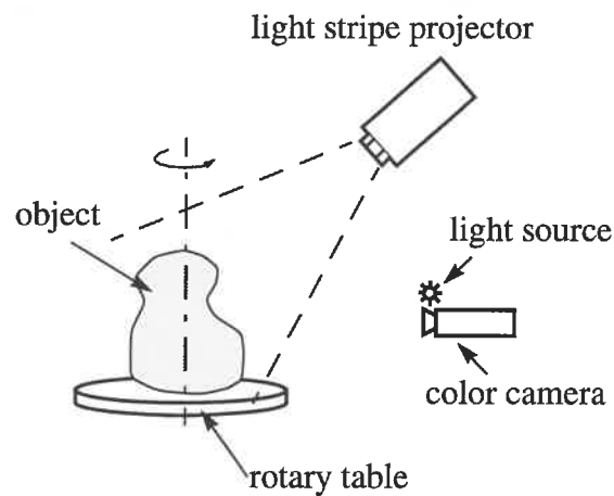
Figure 1 Experimental setup
