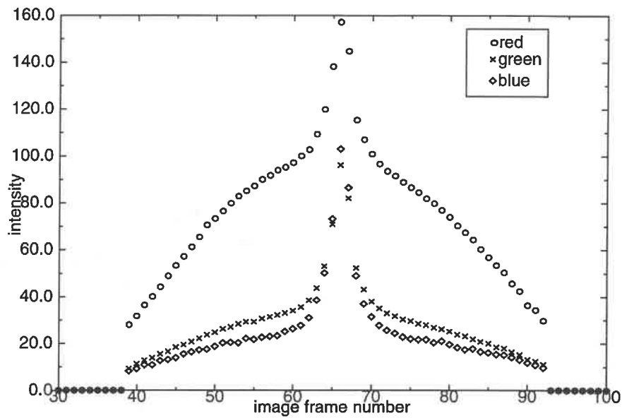
Figure 4 intensity change with strong specularity
