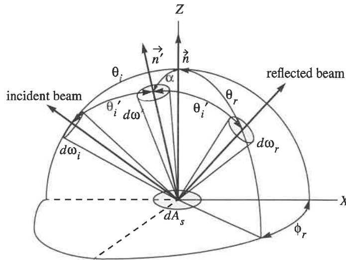
Figure 9 Geometry for Torrance-Sparrow model [22]
