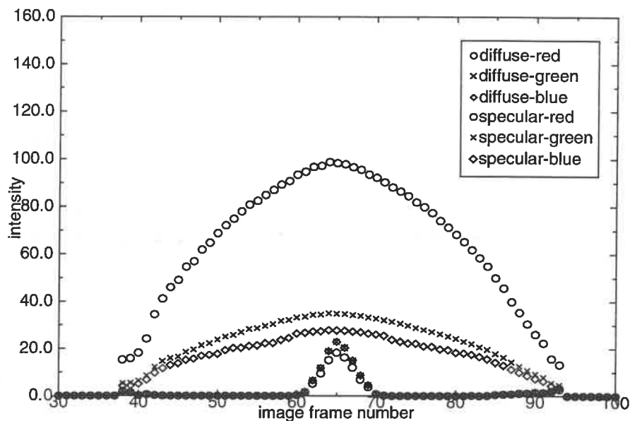
Figure 7 separated reflection component with little specularity
