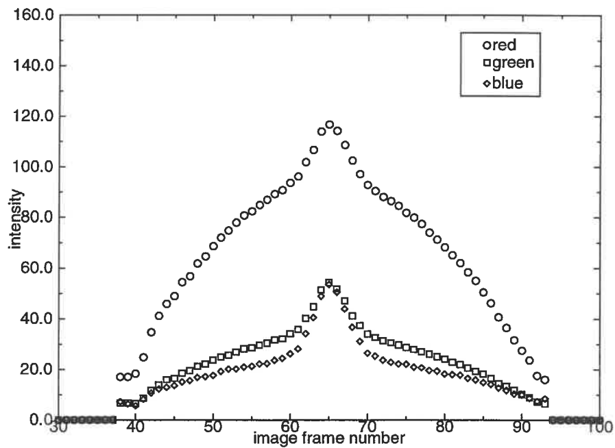
Figure 5 intensity change with little specularity
