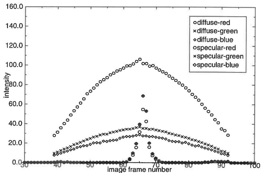
Figure 6 separated reflection components with strong specularity
