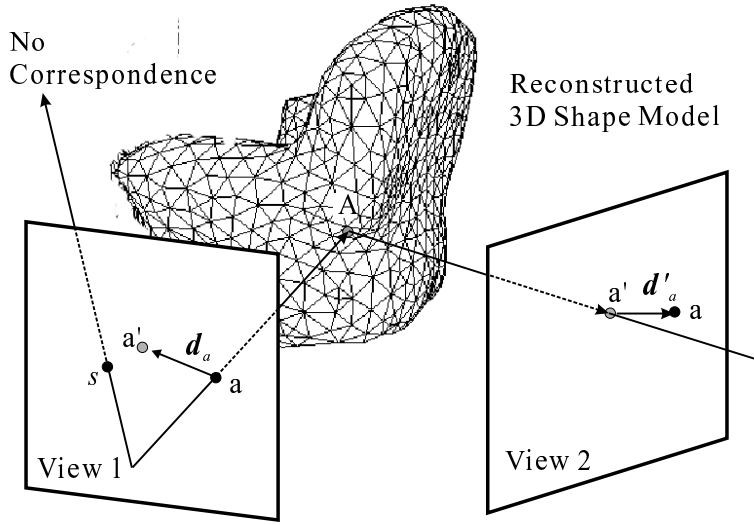
Figure 7: The scheme for making correspondences in accordance with a 3D shape model.
