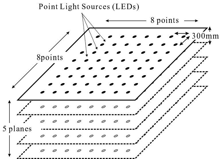
Figure 6: Placement of point light sources for calibration of every camera in the 3D Room.
