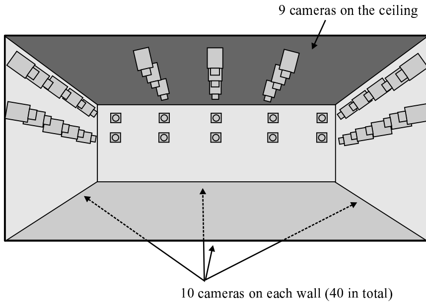
Figure 1: Camera placement in the 3D Room.
