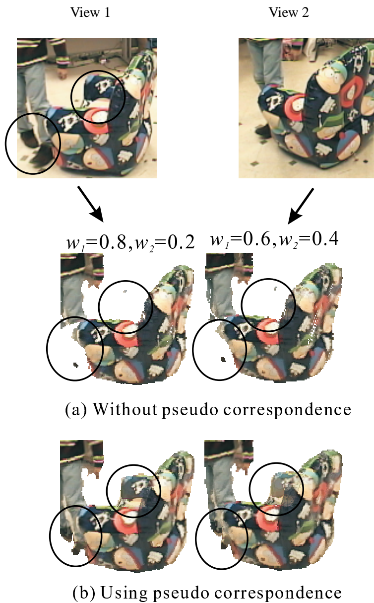
Figure 9: Effect of the pseudo correspondence in view interpolation. If we only have two views, there is no way to compute the correspondences correctly for the occlusion regions in view 1 (circled areas). Therefore the colors in this regions do not exist in the interpolated view images (a). On the other hand, the 3D shape model provides the pseudo corresponding points for the occlusion regions in view 1. Therefore the colors in those regions appear in the interpolated view images (b).
