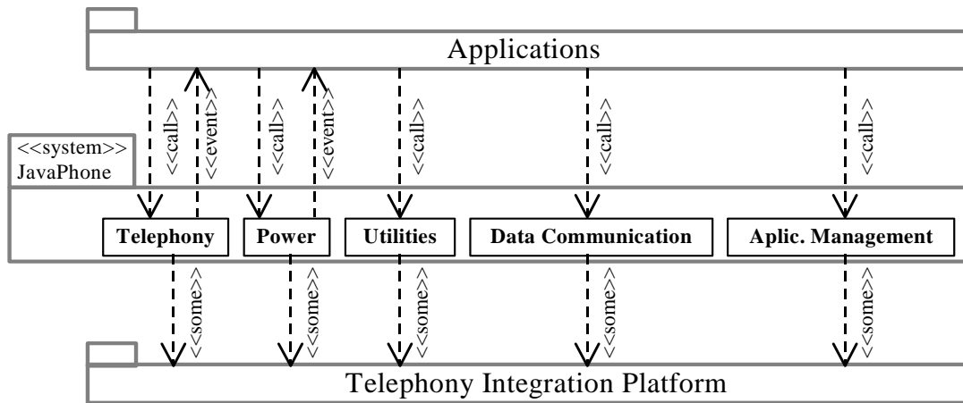
Figure 15: Package diagram corresponding to Figure 14
