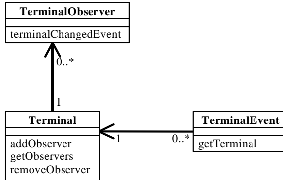
Figure 17: Class diagram for the interfaces defining the event-observer pattern for Terminal
