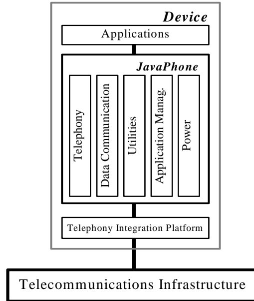
Figure 7: Detailing the domain view of JavaPhone
