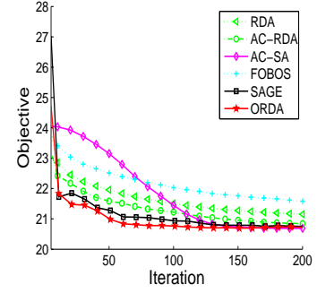
Figure 5.1: Objective values v.s. Iterations. Only the first 200 iterations are plotted for better visualization and the ease of comparisons.
