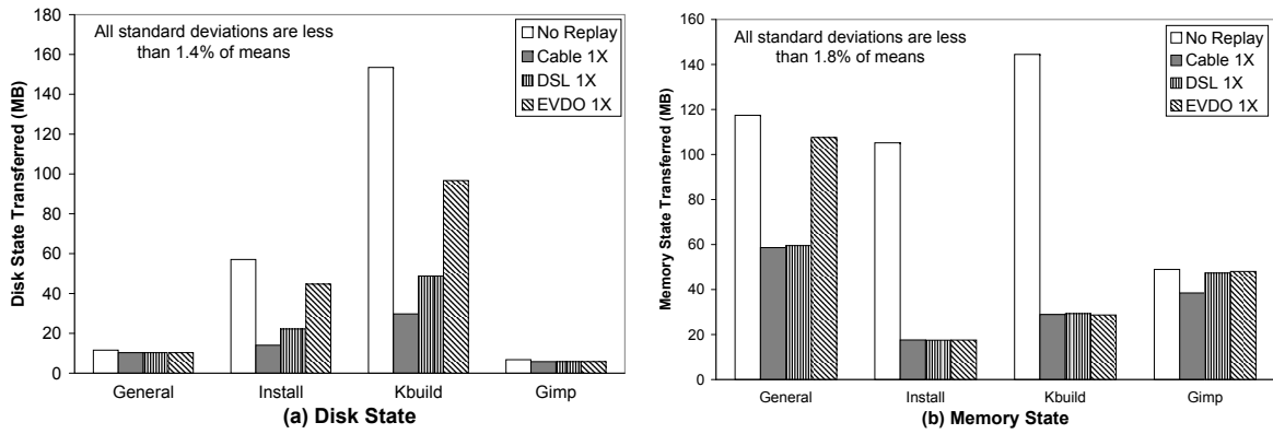
Figure 1: Bytes transferred during replay at native speed
