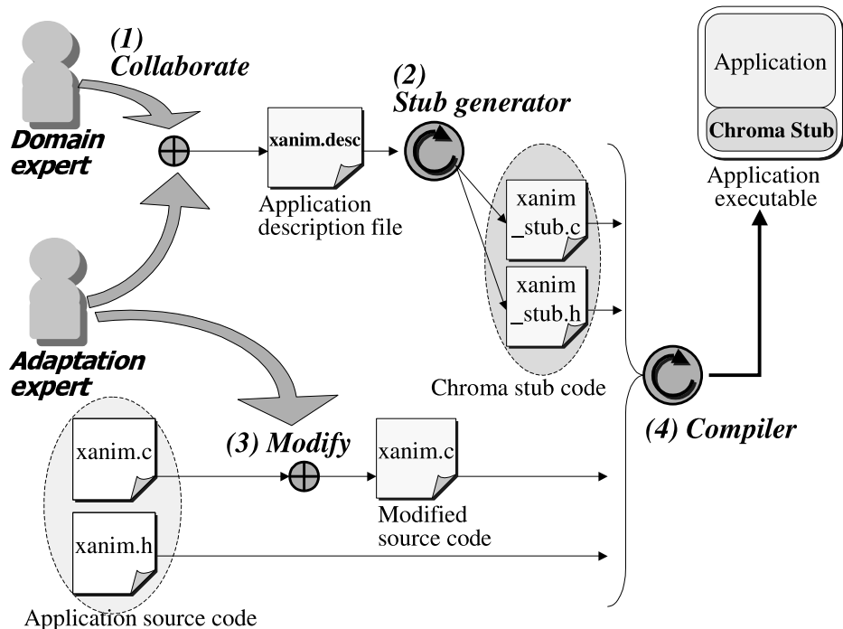
Figure 1: Process for adding adaptation to an application
