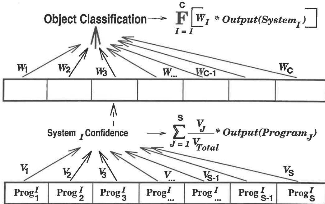
Figure 8: The weights W and V that are trained early in testing.
