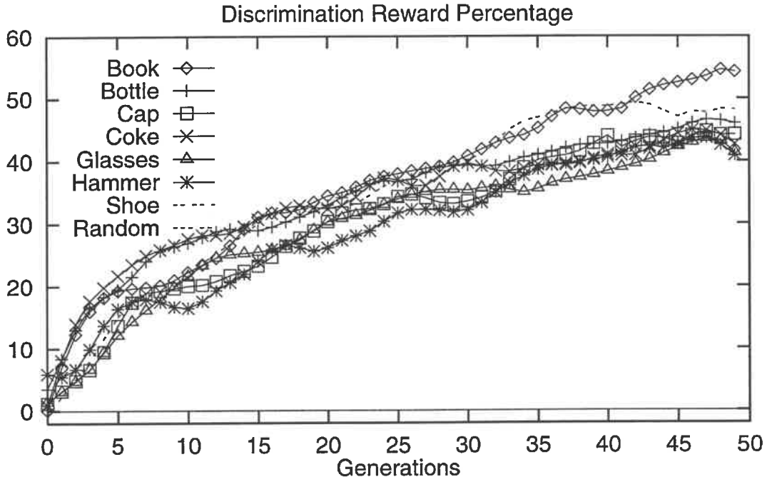
Figure 3: PADO discrimination reward percentage on test images of Set T .
