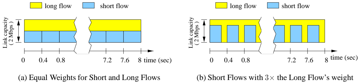
Figure 1: Improving burst delays
