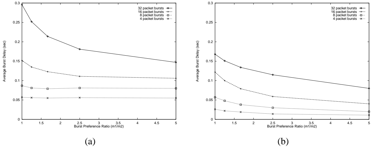
Figure 11: The average burst delay versus BPR for eight flows when the ON-OFF traffic is (a) TCP, and (b) UDP, respectively.
