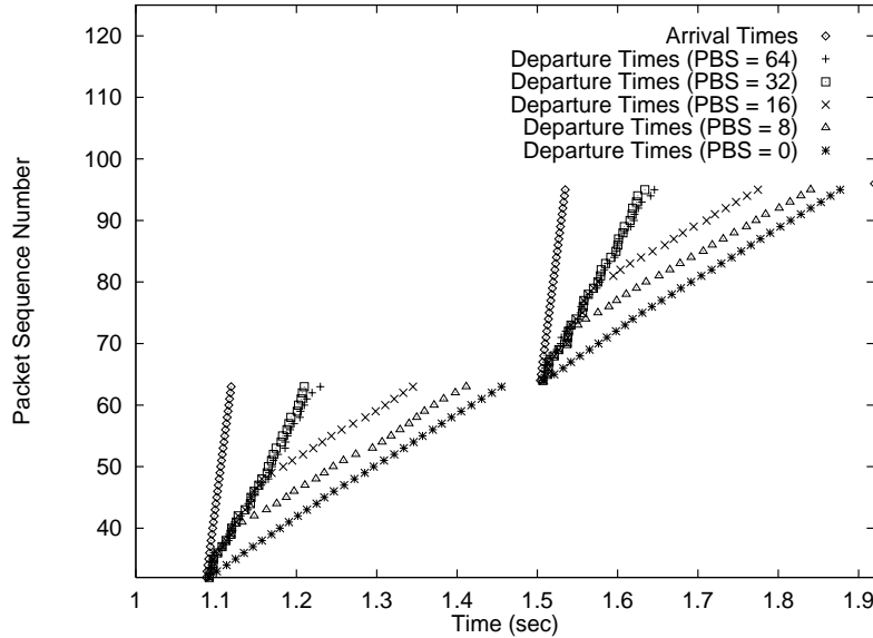
Figure 8: The packet arrival and departure times of a flow, with of 32 packet bursts, for various service curves.
