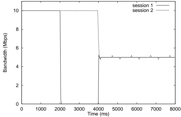
Figure 3: Measured bandwidth of two TCP sessions, startup 2 seconds apart under SCED.
