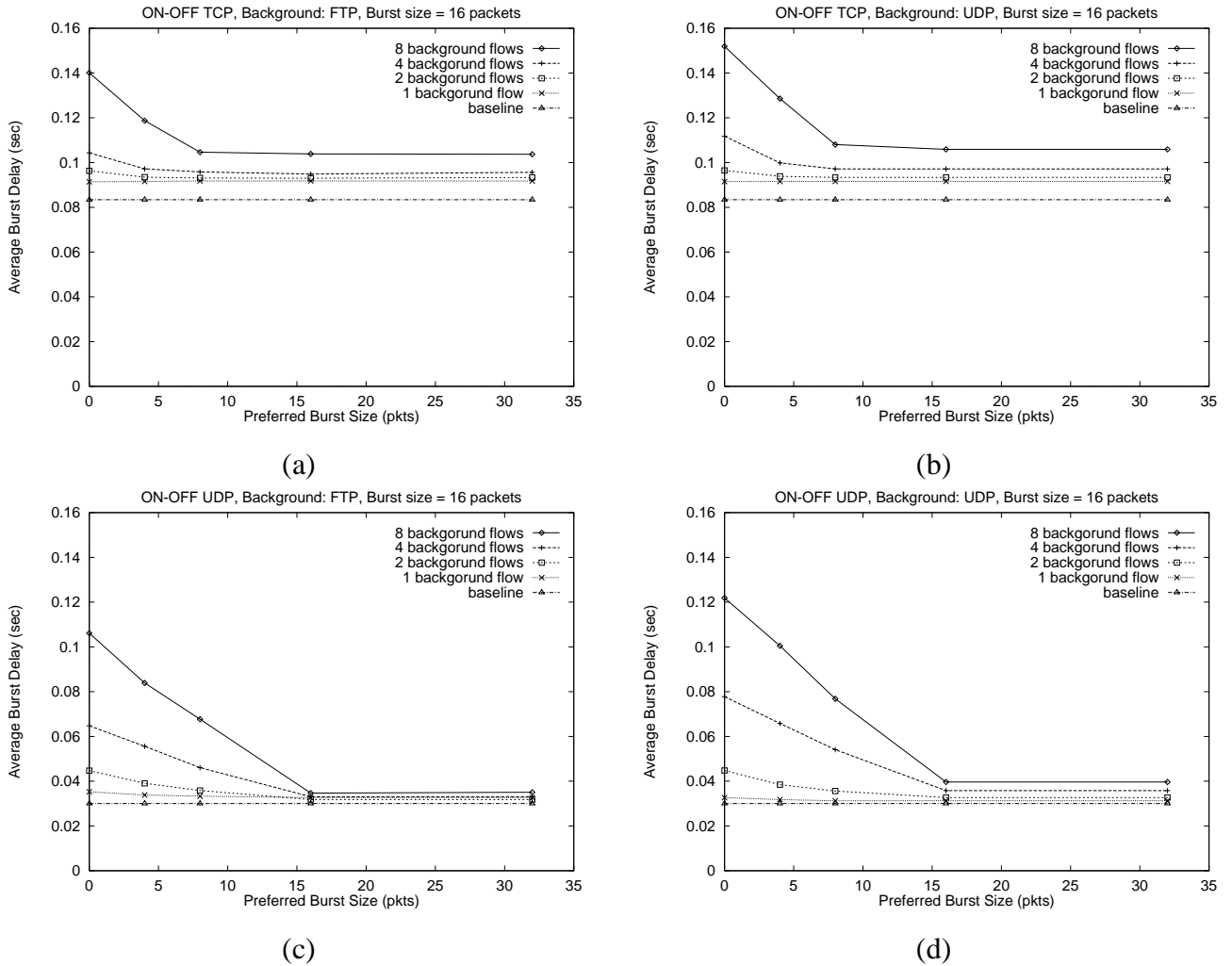
Figure 9: The average burst delay vs PBS for four simulation scenarios, each having 16 flows. Note that the average delay decreases as the PBS increases, up to the burst size of 16 packets.
