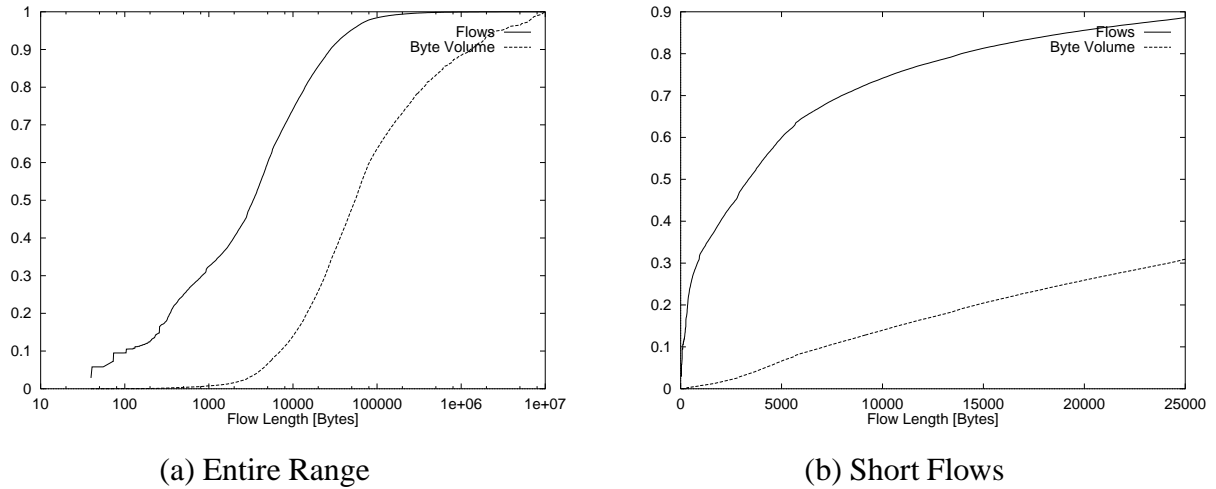
Figure 17: Cumulative probability distribution of flow lengths and their portion of the total byte volume.
