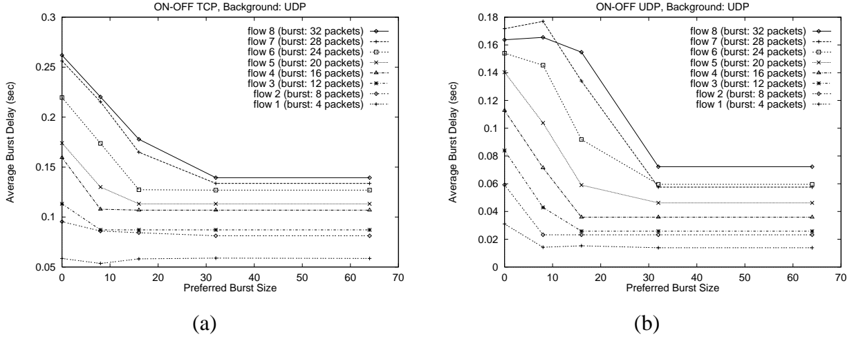
Figure 12: The average burst delay versus PBS for eight flows, with burst sizes between 4 and 32 packets, when the ON-OFF traffic is (a) TCP, and (b) UDP, respectively.
