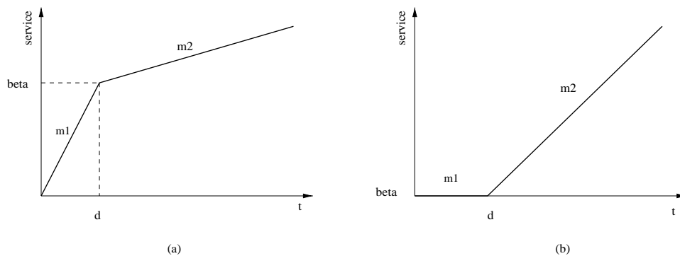
Figure 2: Sample service curves.
