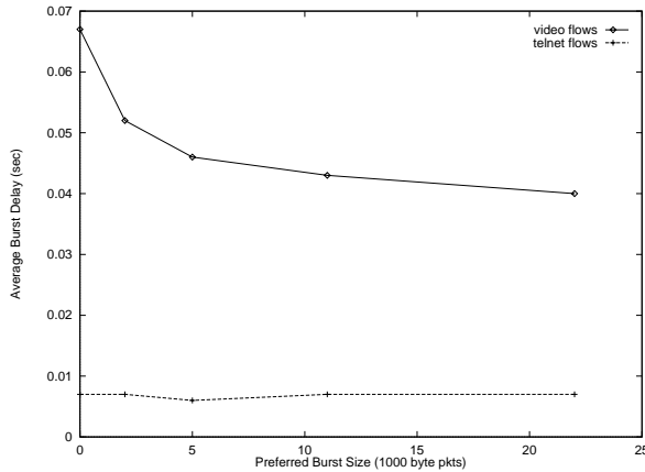
(a) Entire Range
