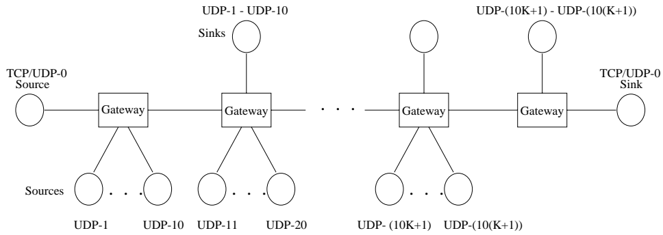
Figure 15: Topology for analyzing the effects of multiple congested links on the throughput of a flow. Each congested link is traversed by ten cross flows (all UDPs).
