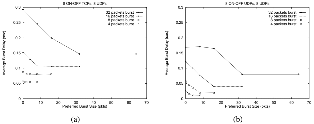
Figure 10: The average burst delay of eight ON-OFF TCP/UDP flows as a function of PBS for various burst sizes.
