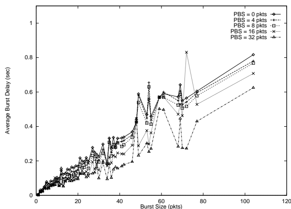
Figure 13: The average burst delay versus burst size for eight ON-OFF TCP flows, which have burst sizes exponentially distributed with a mean of 16 packets. The flows compete with other eight constant-bit-rate UDP flows.
