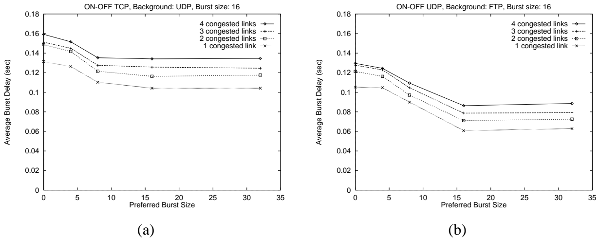
Figure 16: (a) The average burst delay versus PBS as the number of bottleneck links varies. The foreground traffic consists of one ON-OFF TCP. (b) The same experiment when the foreground traffic consists of one ON-OFF UDP.
