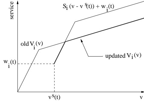
Figure 7: Illustration of the update of the virtual curve.
