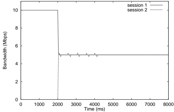
Figure 4: Measured bandwidth of two TCP sessions, startup 2 seconds apart under FSC.
