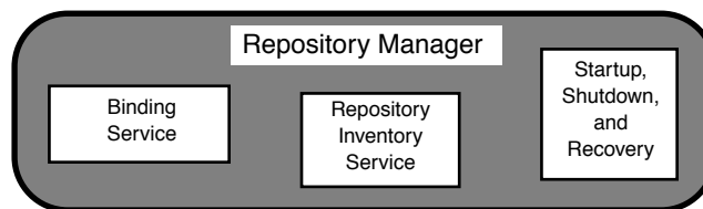
Figure 28. Repository Manager Functional Composition
