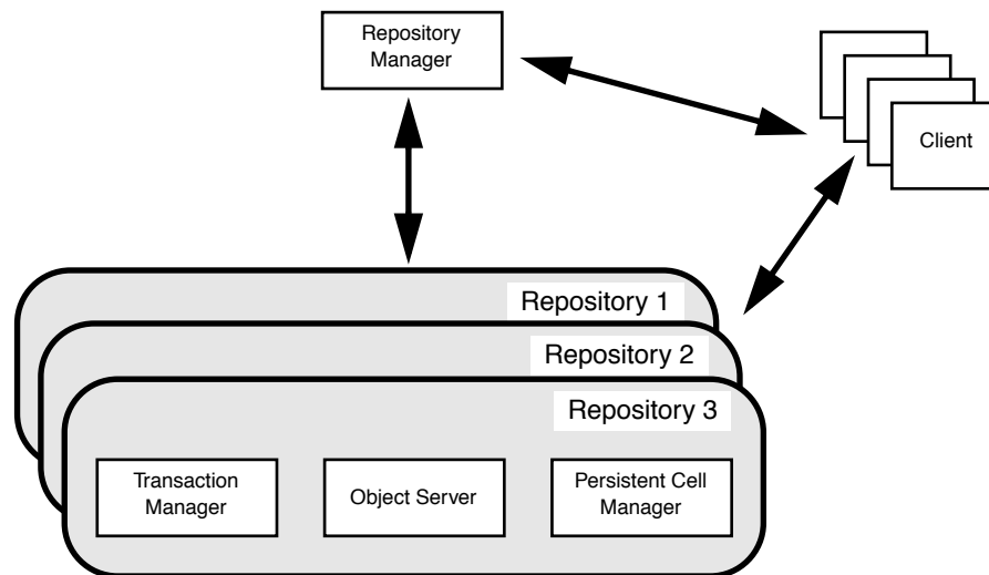
Figure 5. Common Features of the Parameterized Architecture
