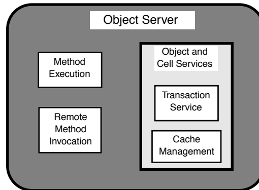
Figure 31. Object Server Functional Composition
