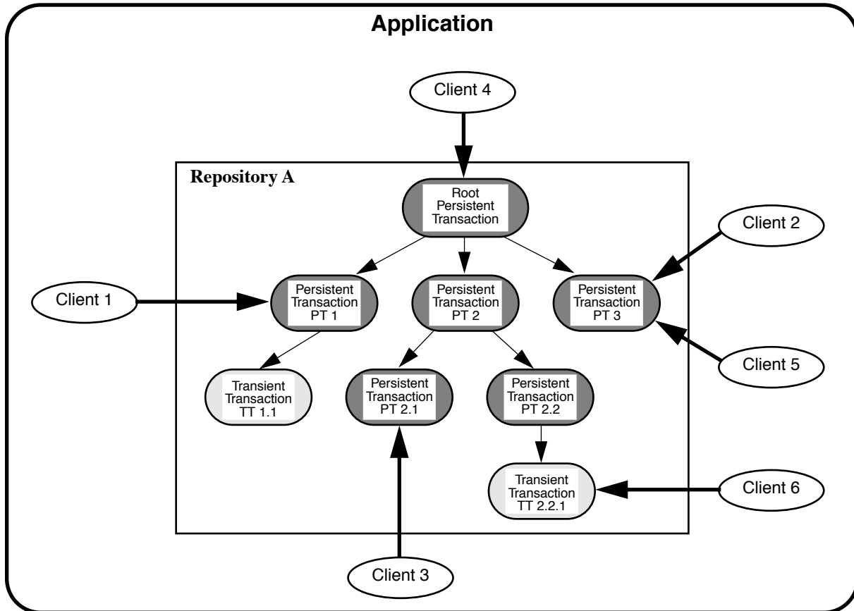
Figure 24. A Transaction Hierarchy in a UFO Repository
