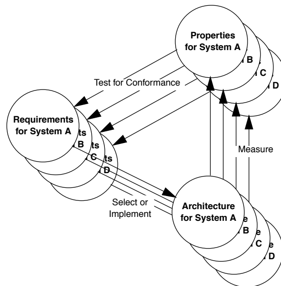
Figure 2. Requirements, Architectures, and Properties for a Class of Systems
