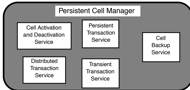
Figure 30. Persistent Cell Manager Functional Composition
