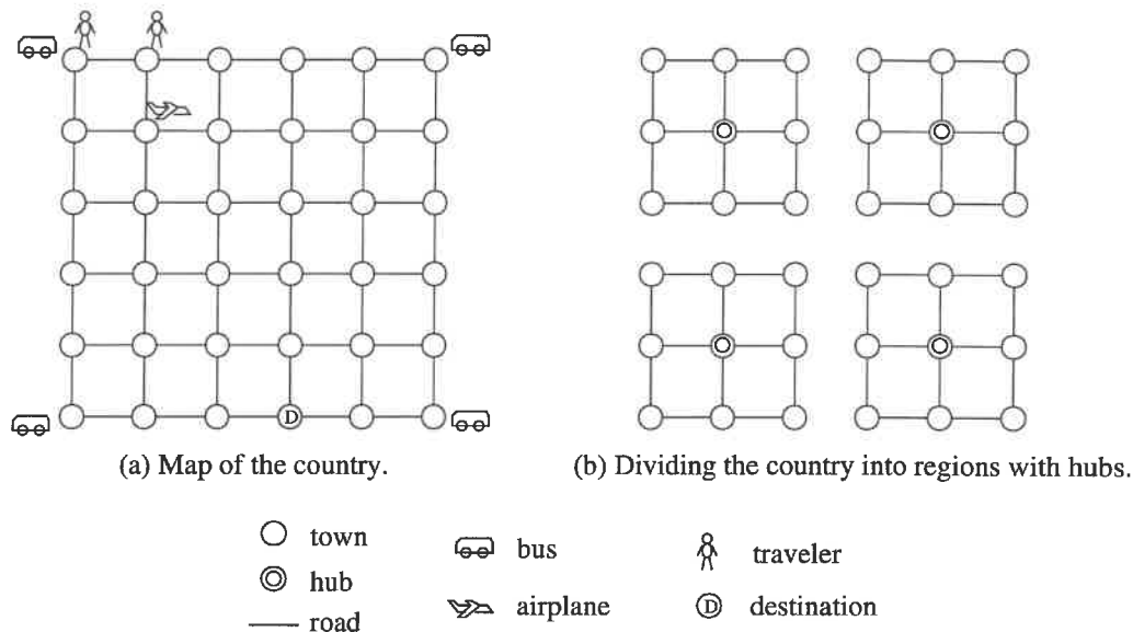
Figure 3: Changing the representation of the Interurban Transportation domain: we simplify planning problems by dividing the country into regions with hubs; the airplane flies only between hubs, whereas the buses deliver people to and from hubs within regions.
