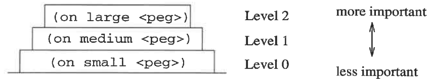
(d) Abstraction hierarchy of predicates generated by ALPINE.
