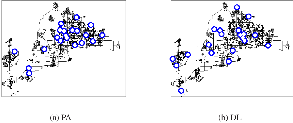
Figure 8.10: Water network sensor placements: (a) when optimizing PA, sensors are concentrated in high population areas. (b) when optimizing DL, sensors are uniformly spread out.
