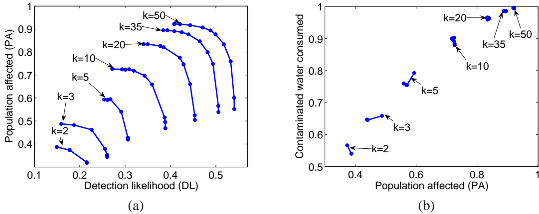
Figure 8.12: (a) Trading off PA and DL. (b) Trading off PA and consumed contaminated water.
