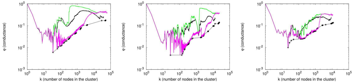
Leighton-Rao: connected clusters (green), disconnected clusters (magenta).
