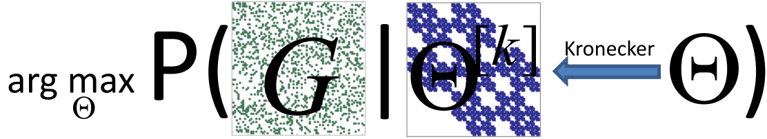
Figure 5.11: Kronecker parameter estimation as an optimization problem. We search over the initiator matrices \Theta (\equiv \mathcal{P}_1) . Using Kronecker multiplication we create probabilistic adjacency matrix \Theta^{[k]} that is of same size as real network G . Now, we evaluate the likelihood by simultaneously traversing and multiplying entries of G and \Theta^{[k]} (see Eq. 5.5). As shown by the figure permutation \sigma plays an important role, as permuting rows and columns of G could make it look more similar to \Theta^{[k]} and thus increase the likelihood.
