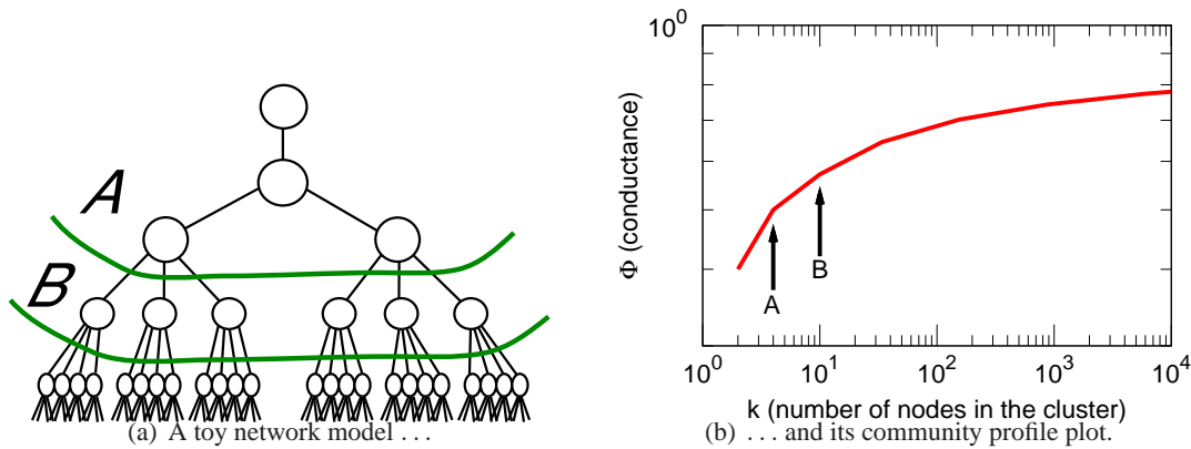
Figure 10.19: Schematic picture of the properties of a network responsible for the upward-sloping community profile plot. (a) This toy model is designed so that the optimal conductance cuts are achieved by cutting nodes from the top of the tree. (b) The minimum of the NCP plot is achieved by cutting the single top node, and then larger and larger cuts have gradually worse and worse conductance values.
