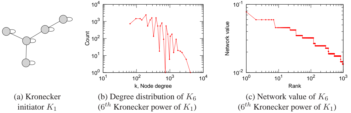
Figure 5.5: The “staircase” effect. Kronecker initiator and the degree distribution and network value plot for the 6 th Kronecker power of the initiator. Notice the non-smoothness of the curves.
