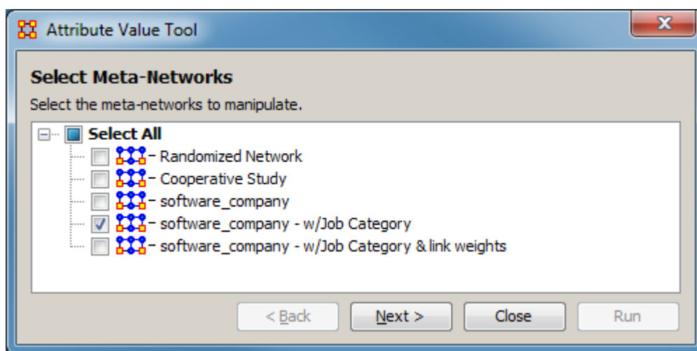
Select Meta-Networks
