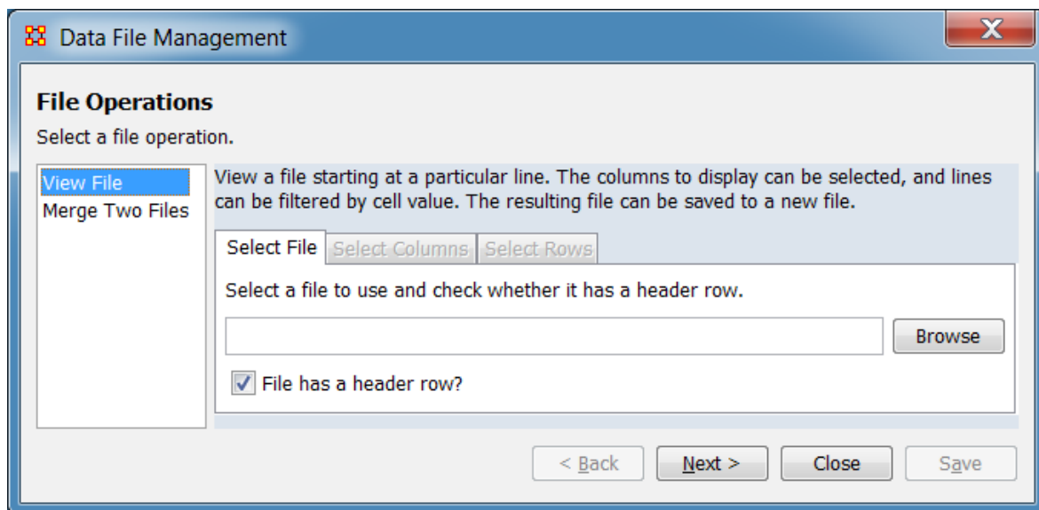
File Operations
