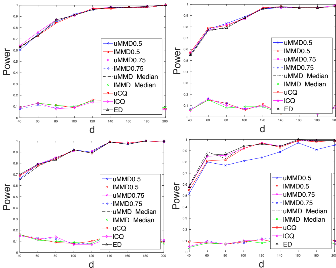
Figure 10.1: Power vs Dimension when P, Q are mean-shifted Normal (top left), Laplace (top right), Betas (bottom left) or Mixture (bottom right plot) distributions.
