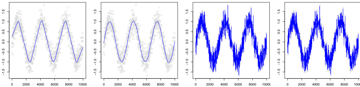
Figure 9.9: Visualization of trend filtering estimates for the experiments in Figures 9.7, 9.10. The estimates were trained on n = 10,000 points from an underlying sinusoidal curve (but the above plots have been downsampled to 1000 points for visibility). The two left panels show the fits for k = 1, 2 , respectively, in the high regularization regime, where \lambda is near \lambda_{\max} . The specialized ADMM approach outperforms PDIP (and shown are the ADMM fits). The two right panels show the fits for k = 1, 2 , respectively, in the low regularization regime, with \lambda = 10^{-5}\lambda_{\max} . PDIP converges faster than ADMM (and shown are the PDIP fits), but this is not a statistically reasonable regime for trend estimation.
