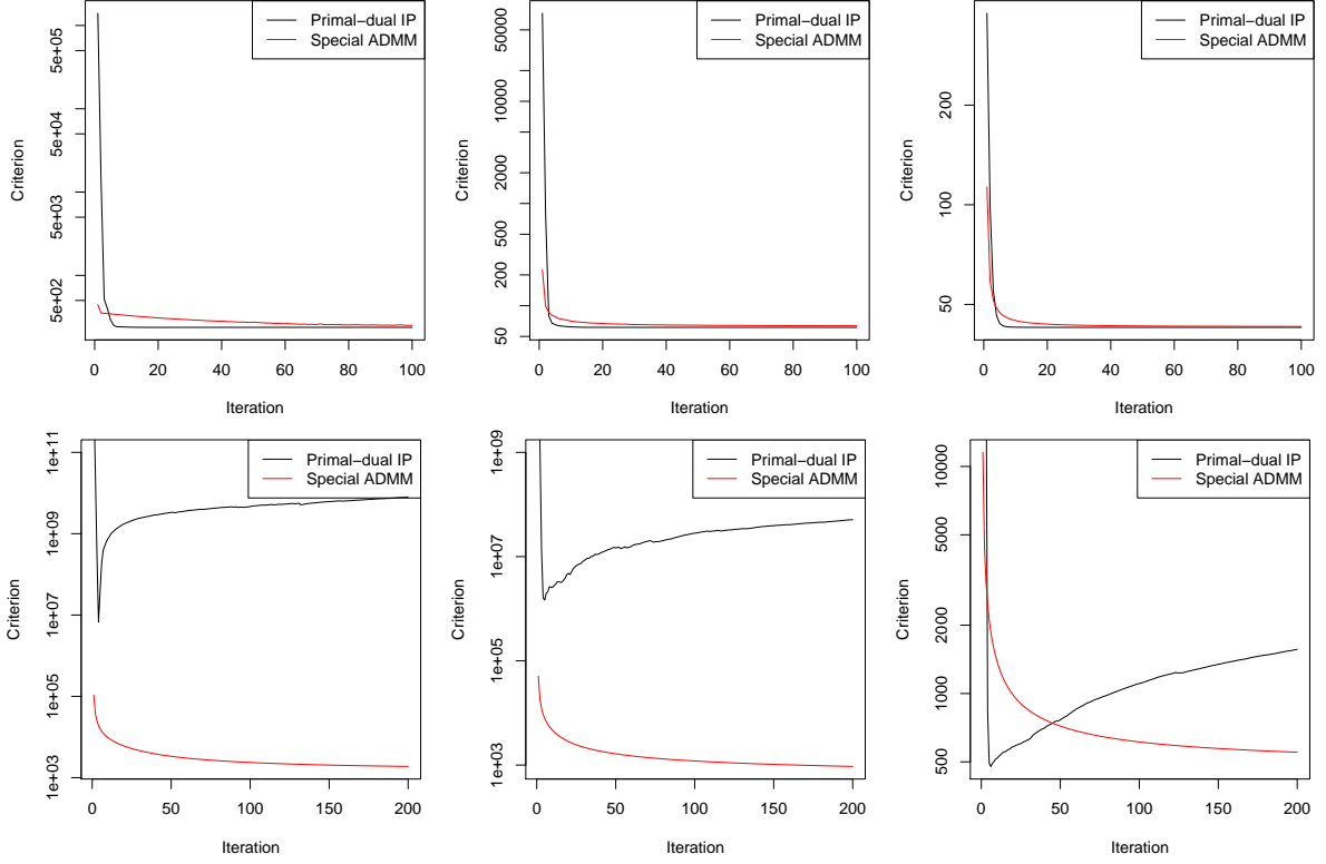
Figure 9.14: Convergence plots for (k = 3) : achieved criterion values across iterations of ADMM and PDIP, with the same layout as in Figures 9.5 and 9.8, except that the first row uses n = 1000 points, and the second row n = 10,000 points. Both algorithms comfortably converge when n = 1000 . However, PDIP encounters serious difficulties when n = 10,000 , reminiscent of its behavior for k = 2 but when n = 100,000 (see Figure 9.8). In all cases, the specialized ADMM algorithm demonstrates a strong and steady convergence behavior.
