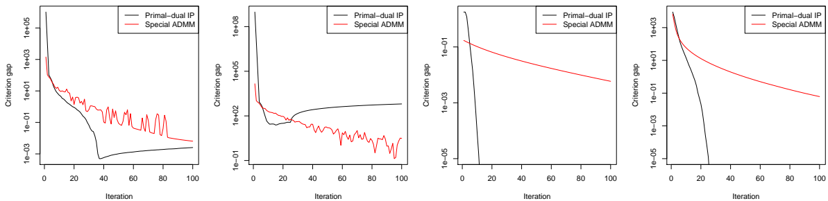
Figure 9.6: Convergence gaps for k = 1 : achieved criterion value minus the optimum value across iterations of ADMM and PDIP. Here the optimum value was defined as smallest achieved criterion value over 5000 iterations of either algorithm. The first two plots are for \lambda near \lambda_{\max} , with n = 10,000 and n = 100,000 points, respectively. In this high regularization regime, ADMM fares better for large n . The last two plots are for \lambda = 10^{-5}\lambda_{\max} , with n = 10,000 and n = 100,000 , respectively. Now in this low regularization regime, PDIP converges at what appears to be a second-order rate, and ADMM does not. However, these small values of \lambda are not statistically interesting in the context of the example, as they yield grossly overfit trend estimates of the underlying sinusoidal curve.
